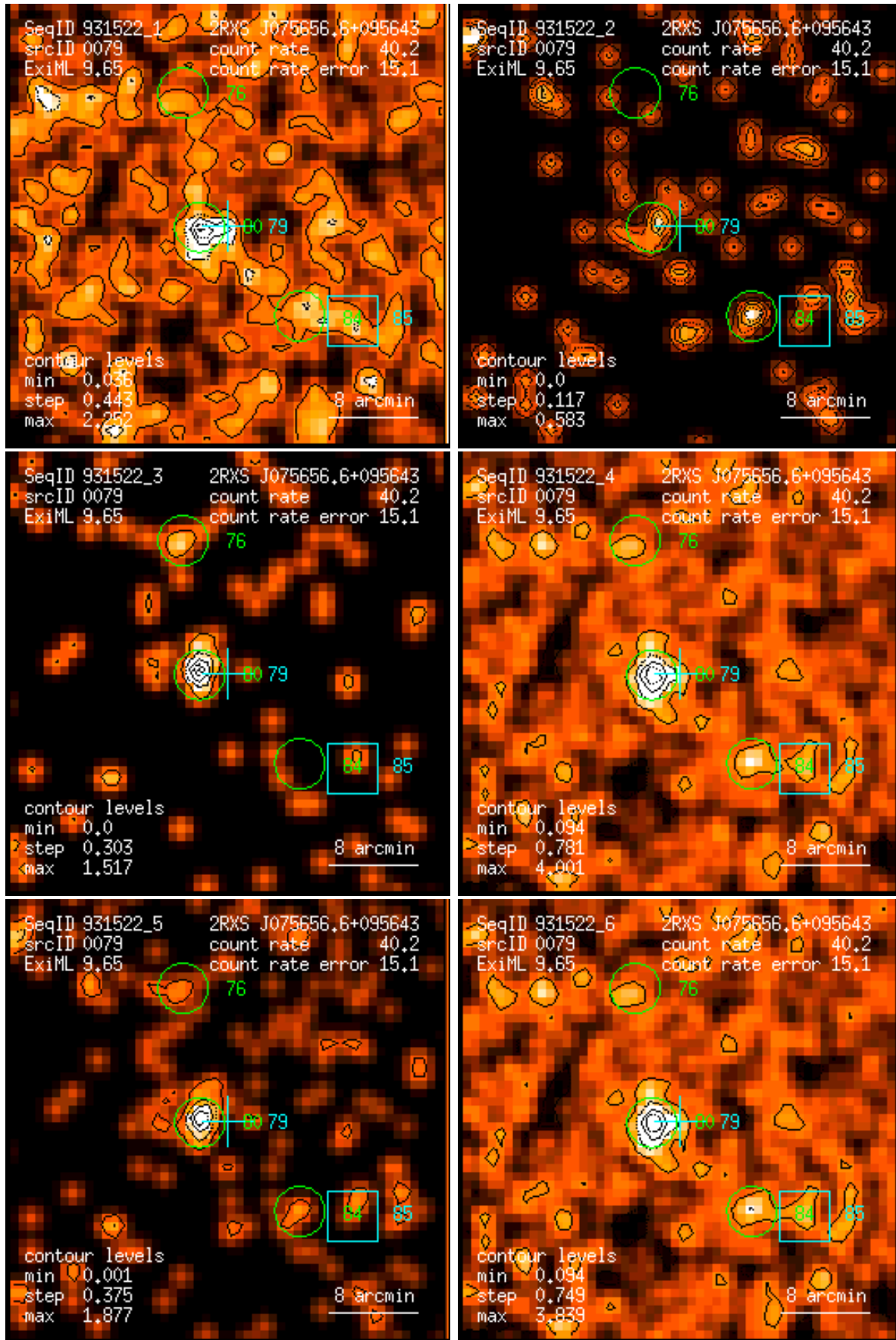
Figure 79: RASS 931522: detection 0079: band rate images, Gaussian filter: (1) PSPC channels 11 – 41, (2) 52 – 90, (3) 91 – 201, (4) 11 – 235, (5) 52 – 201, (6) 11 – 201. Broad band rates in counts/ks. Band rate contour levels in counts/ks/arcmin 2 .
