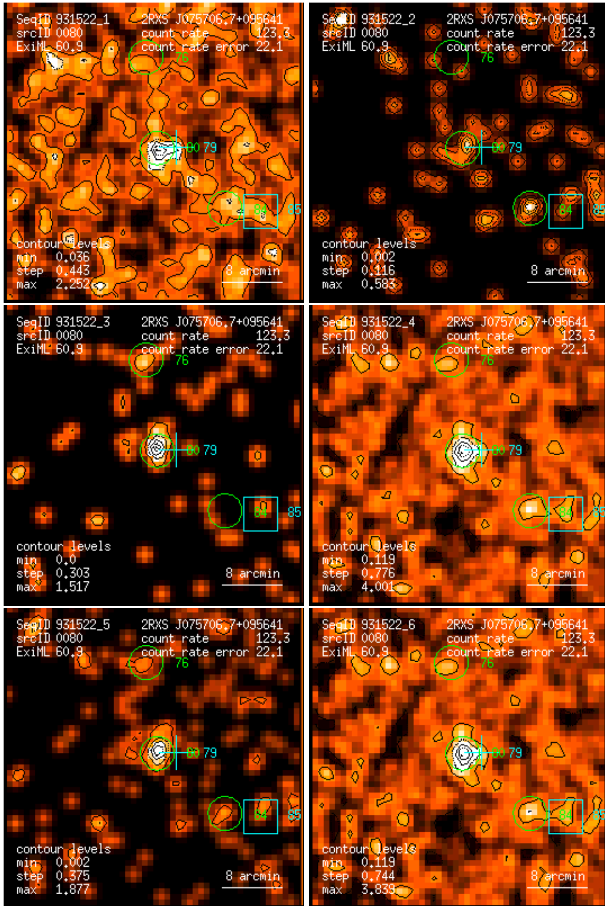
Figure 80: RASS 931522: detection 0080: band rate images, Gaussian filter: (1) PSPC channels 11 – 41, (2) 52 – 90, (3) 91 – 201, (4) 11 – 235, (5) 52 – 201, (6) 11 – 201. Broad band rates in counts/ks. Band rate contour levels in counts/ks/arcmin 2 .
