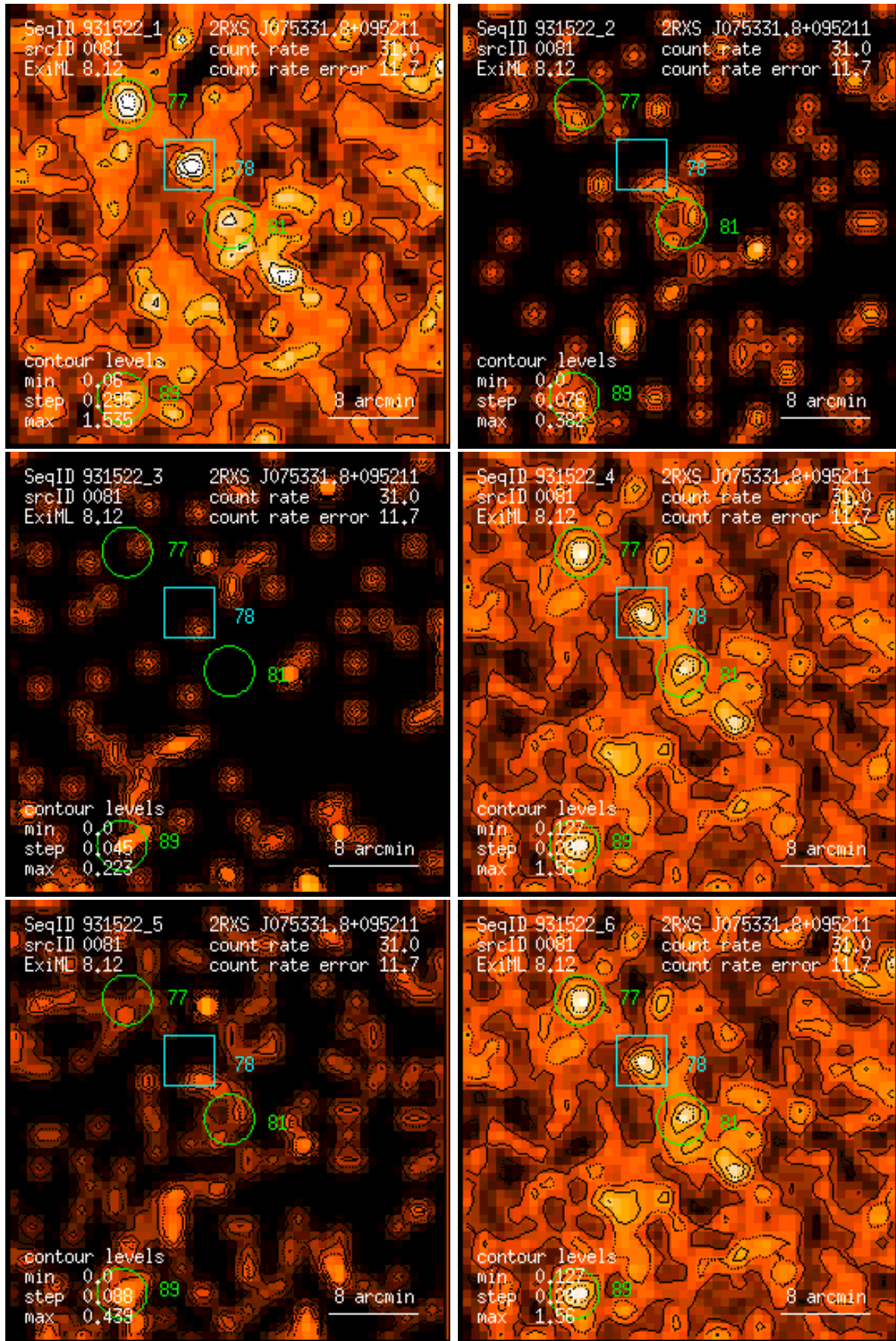
Figure 81: RASS 931522: detection 0081: band rate images, Gaussian filter: (1) PSPC channels 11 – 41, (2) 52 – 90, (3) 91 – 201, (4) 11 – 235, (5) 52 – 201, (6) 11 – 201. Broad band rates in counts/ks. Band rate contour levels in counts/ks/arcmin 2 .
