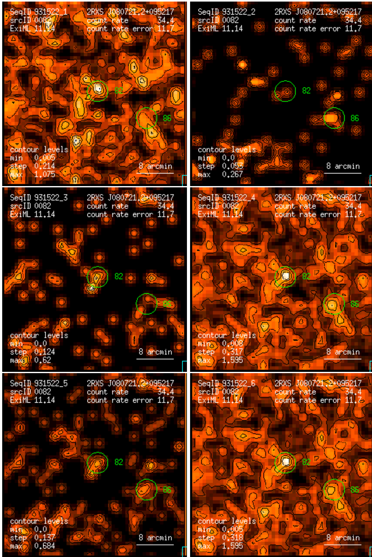
Figure 82: RASS 931522: detection 0082: band rate images, Gaussian filter: (1) PSPC channels 11 – 41, (2) 52 – 90, (3) 91 – 201, (4) 11 – 235, (5) 52 – 201, (6) 11 – 201. Broad band rates in counts/ks. Band rate contour levels in counts/ks/arcmin 2 .
