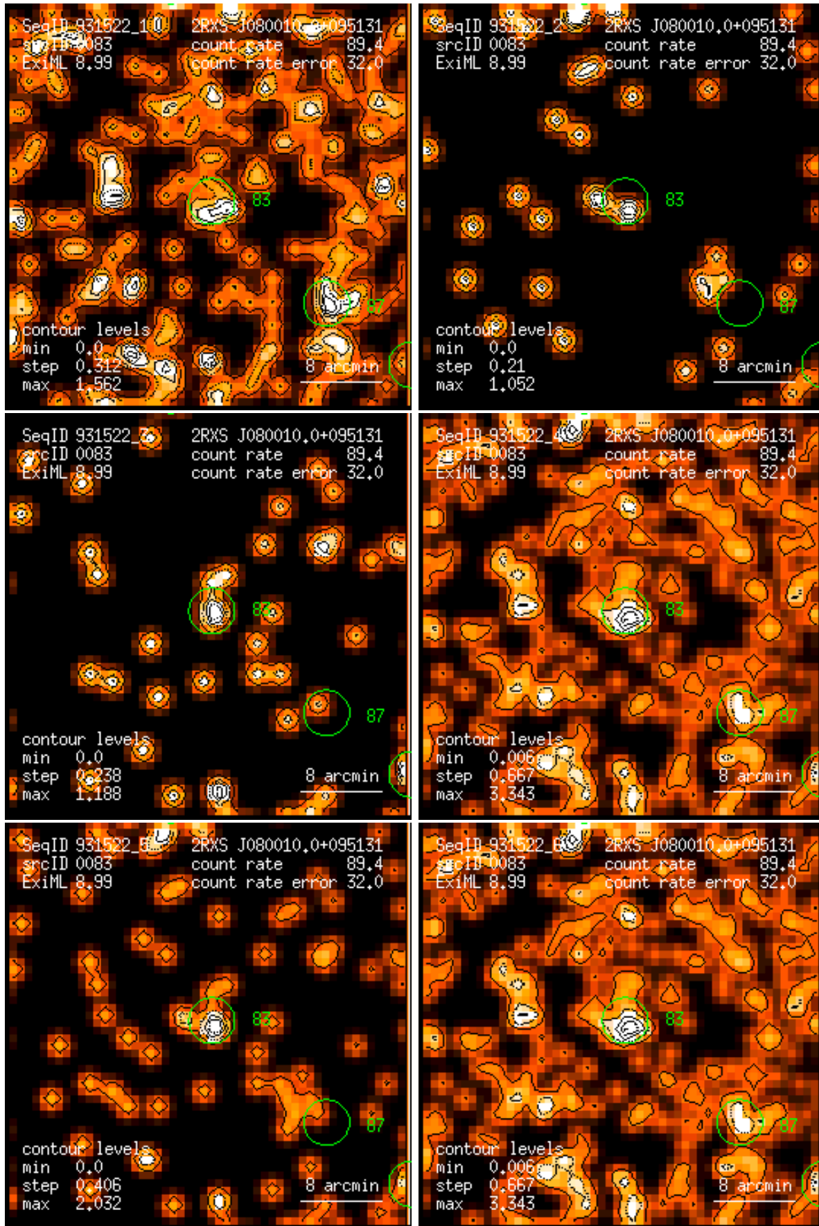
Figure 83: RASS 931522: detection 0083: band rate images, Gaussian filter: (1) PSPC channels 11 – 41, (2) 52 – 90, (3) 91 – 201, (4) 11 – 235, (5) 52 – 201, (6) 11 – 201. Broad band rates in counts/ks. Band rate contour levels in counts/ks/arcmin 2 .
