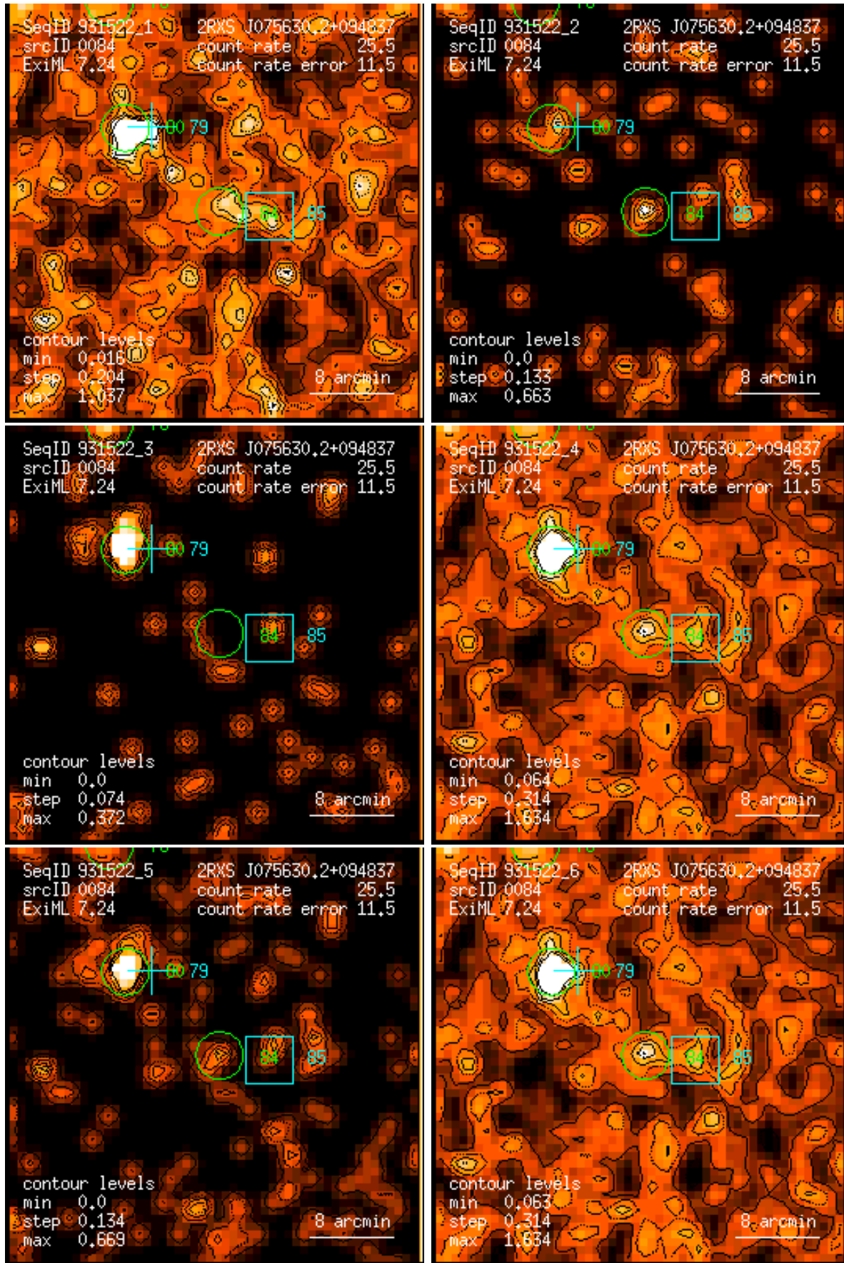
Figure 84: RASS 931522: detection 0084: band rate images, Gaussian filter: (1) PSPC channels 11 – 41, (2) 52 – 90, (3) 91 – 201, (4) 11 – 235, (5) 52 – 201, (6) 11 – 201. Broad band rates in counts/ks. Band rate contour levels in counts/ks/arcmin 2 .
