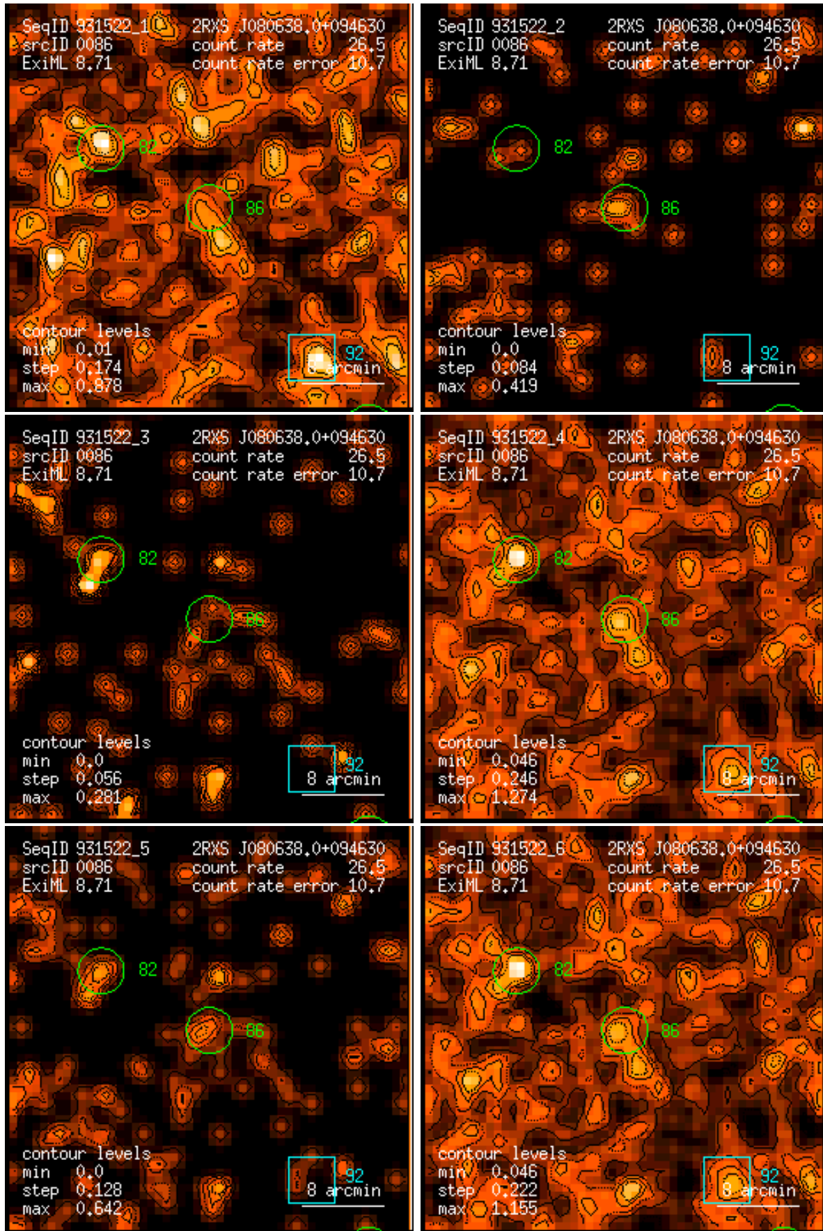
Figure 86: RASS 931522: detection 0086: band rate images, Gaussian filter: (1) PSPC channels 11 – 41, (2) 52 – 90, (3) 91 – 201, (4) 11 – 235, (5) 52 – 201, (6) 11 – 201. Broad band rates in counts/ks. Band rate contour levels in counts/ks/arcmin 2 .
