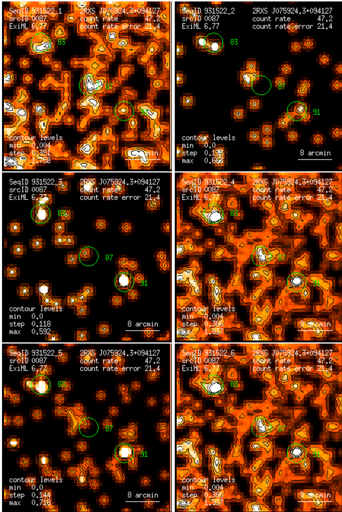
Figure 87: RASS 931522: detection 0087: band rate images, Gaussian filter: (1) PSPC channels 11 – 41, (2) 52 – 90, (3) 91 – 201, (4) 11 – 235, (5) 52 – 201, (6) 11 – 201. Broad band rates in counts/ks. Band rate contour levels in counts/ks/arcmin 2 .
