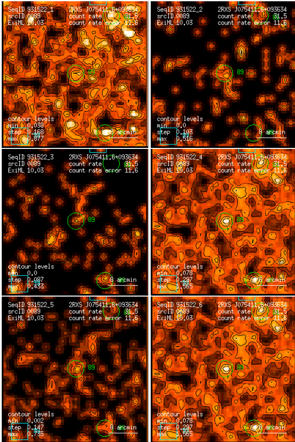
Figure 89: RASS 931522: detection 0089: band rate images, Gaussian filter: (1) PSPC channels 11 – 41, (2) 52 – 90, (3) 91 – 201, (4) 11 – 235, (5) 52 – 201, (6) 11 – 201. Broad band rates in counts/ks. Band rate contour levels in counts/ks/arcmin 2 .
