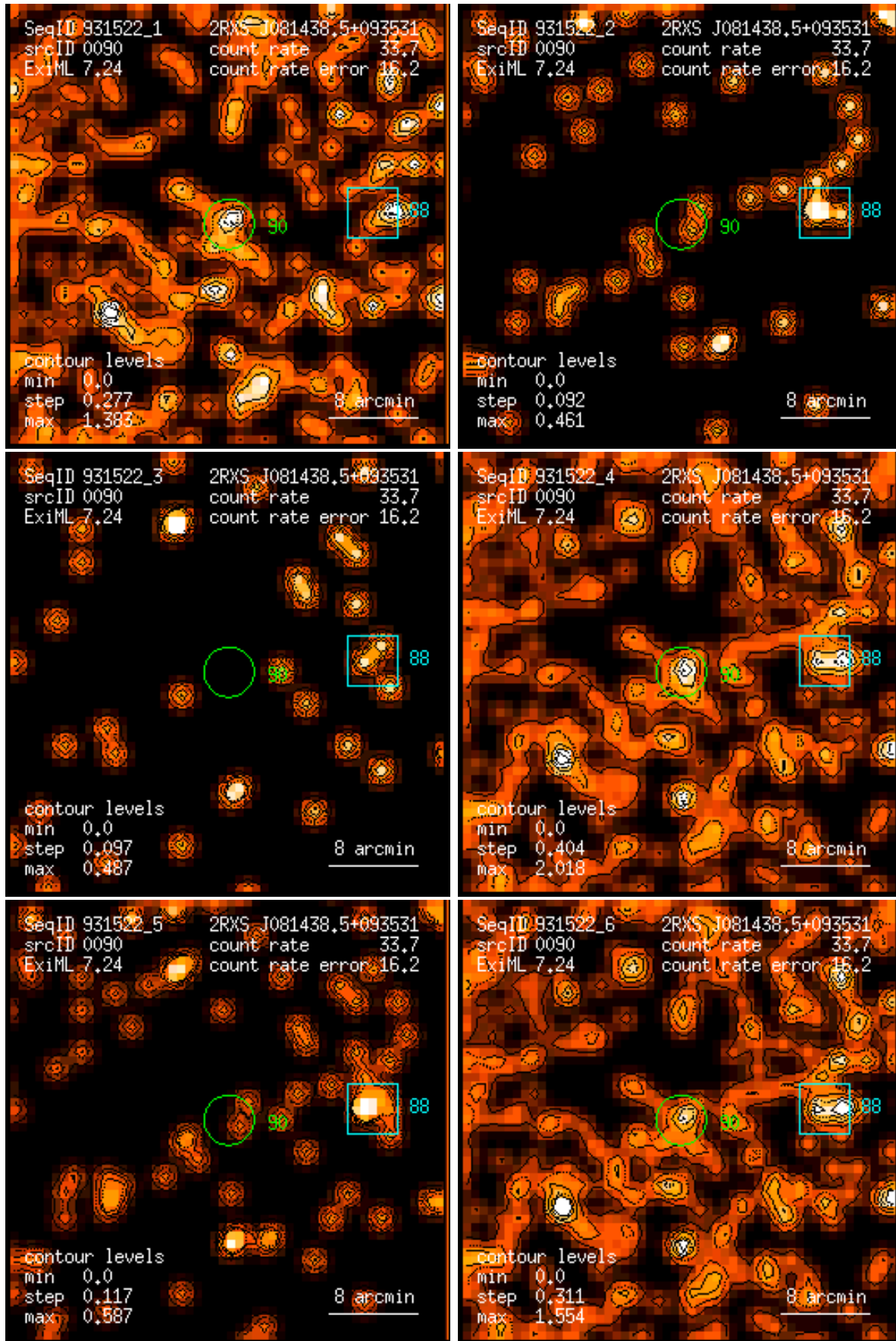
Figure 90: RASS 931522: detection 0090: band rate images, Gaussian filter: (1) PSPC channels 11 – 41, (2) 52 – 90, (3) 91 – 201, (4) 11 – 235, (5) 52 – 201, (6) 11 – 201. Broad band rates in counts/ks. Band rate contour levels in counts/ks/arcmin 2 .
