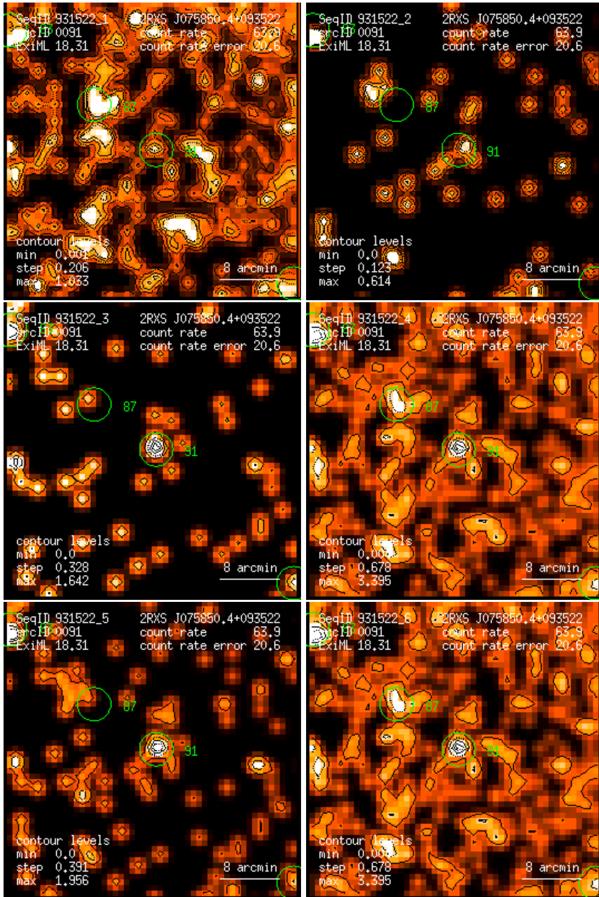
Figure 91: RASS 931522: detection 0091: band rate images, Gaussian filter: (1) PSPC channels 11 – 41, (2) 52 – 90, (3) 91 – 201, (4) 11 – 235, (5) 52 – 201, (6) 11 – 201. Broad band rates in counts/ks. Band rate contour levels in counts/ks/arcmin 2 .
