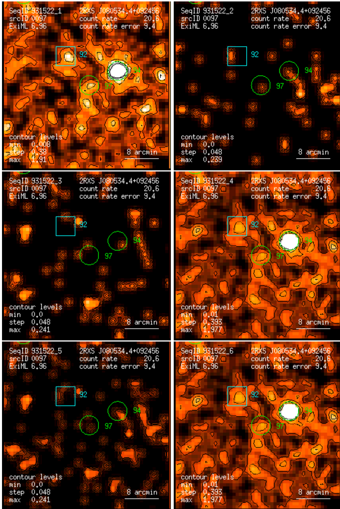
Figure 97: RASS 931522: detection 0097: band rate images, Gaussian filter: (1) PSPC channels 11 – 41, (2) 52 – 90, (3) 91 – 201, (4) 11 – 235, (5) 52 – 201, (6) 11 – 201. Broad band rates in counts/ks. Band rate contour levels in counts/ks/arcmin 2 .
