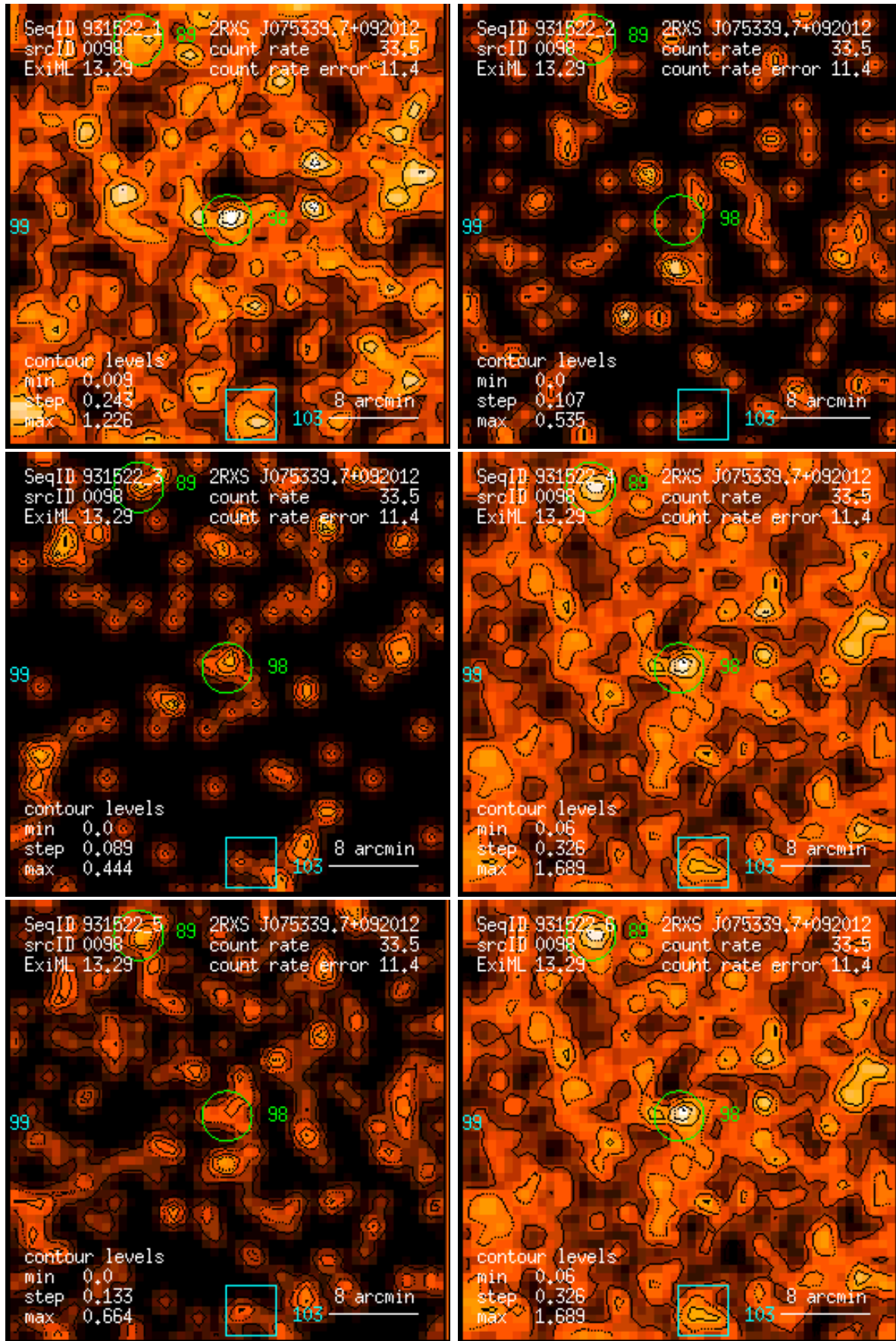
Figure 98: RASS 931522: detection 0098: band rate images, Gaussian filter: (1) PSPC channels 11 – 41, (2) 52 – 90, (3) 91 – 201, (4) 11 – 235, (5) 52 – 201, (6) 11 – 201. Broad band rates in counts/ks. Band rate contour levels in counts/ks/arcmin 2 .
