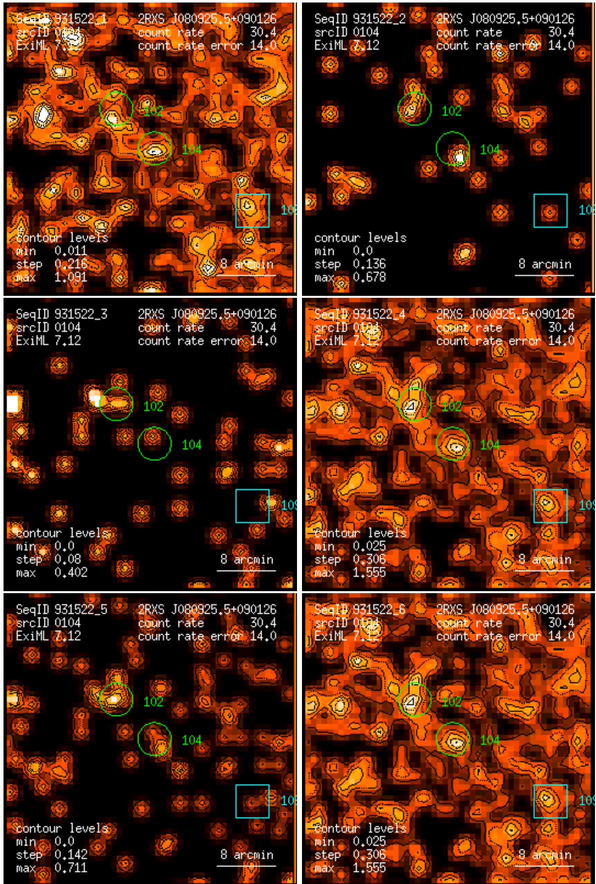
Figure 104: RASS 931522: detection 0104: band rate images, Gaussian filter: (1) PSPC channels 11 – 41, (2) 52 – 90, (3) 91 – 201, (4) 11 – 235, (5) 52 – 201, (6) 11 – 201. Broad band rates in counts/ks. Band rate contour levels in counts/ks/arcmin 2 .
