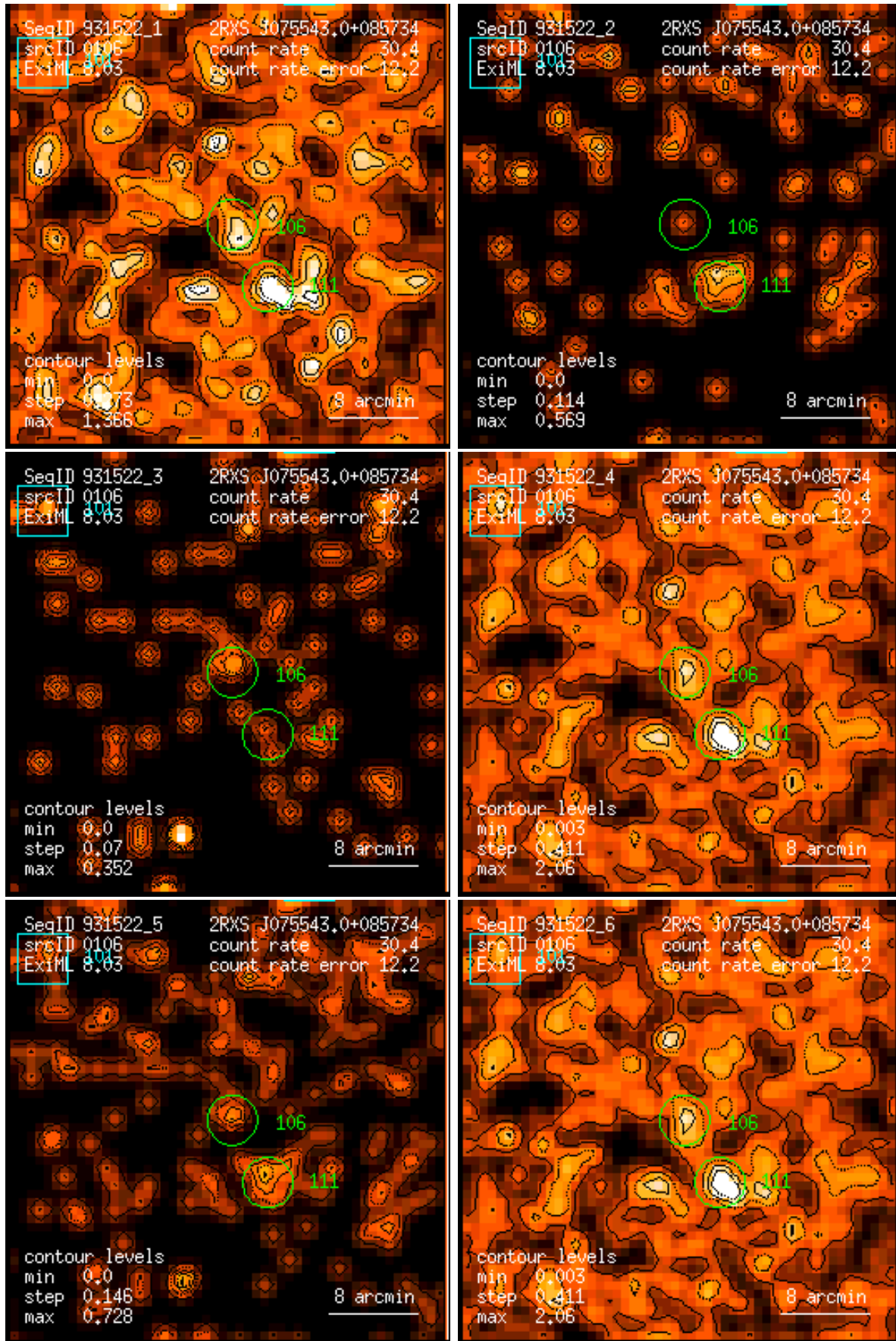
Figure 106: RASS 931522: detection 0106: band rate images, Gaussian filter: (1) PSPC channels 11 – 41, (2) 52 – 90, (3) 91 – 201, (4) 11 – 235, (5) 52 – 201, (6) 11 – 201. Broad band rates in counts/ks. Band rate contour levels in counts/ks/arcmin 2 .
