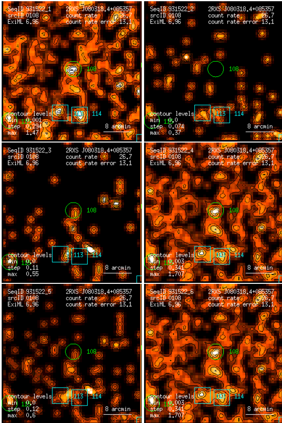
Figure 108: RASS 931522: detection 0108: band rate images, Gaussian filter: (1) PSPC channels 11 – 41, (2) 52 – 90, (3) 91 – 201, (4) 11 – 235, (5) 52 – 201, (6) 11 – 201. Broad band rates in counts/ks. Band rate contour levels in counts/ks/arcmin 2 .
