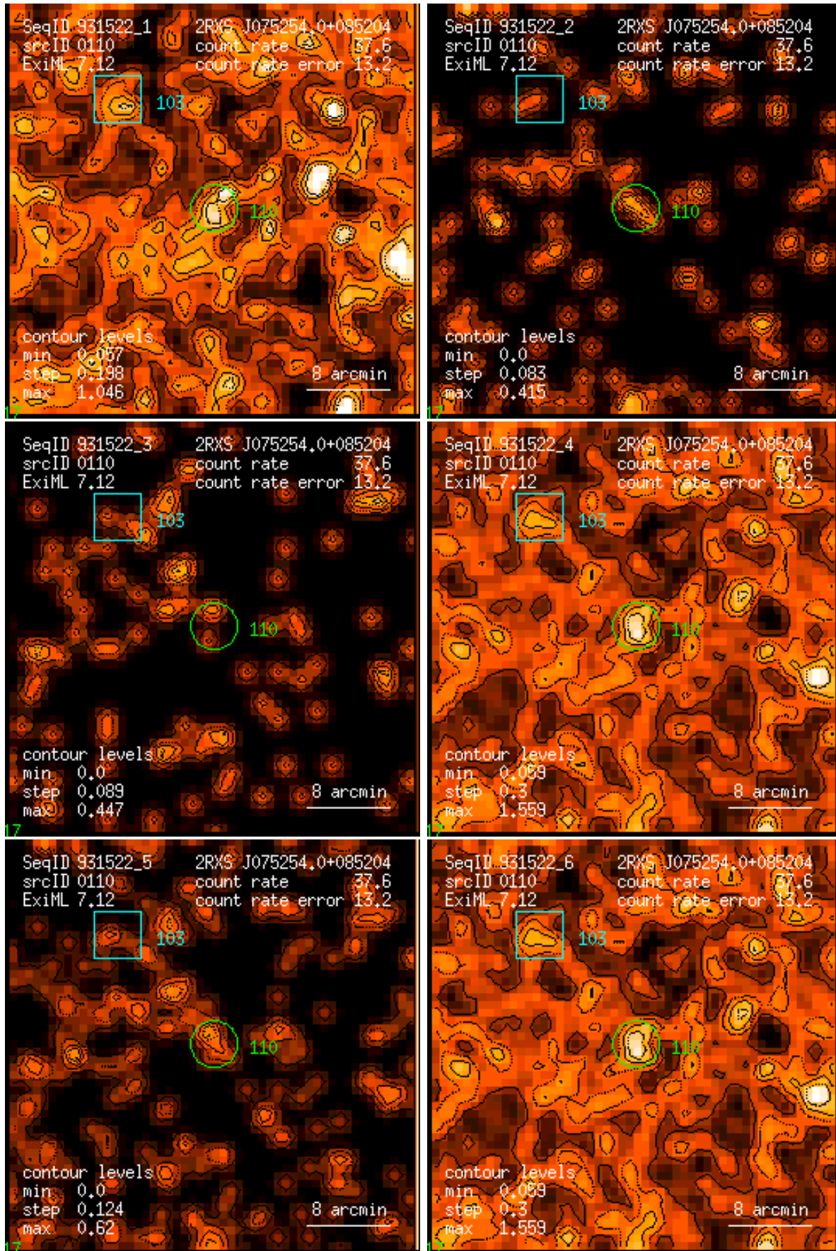
Figure 110: RASS 931522: detection 0110: band rate images, Gaussian filter: (1) PSPC channels 11 – 41, (2) 52 – 90, (3) 91 – 201, (4) 11 – 235, (5) 52 – 201, (6) 11 – 201. Broad band rates in counts/ks. Band rate contour levels in counts/ks/arcmin 2 .
