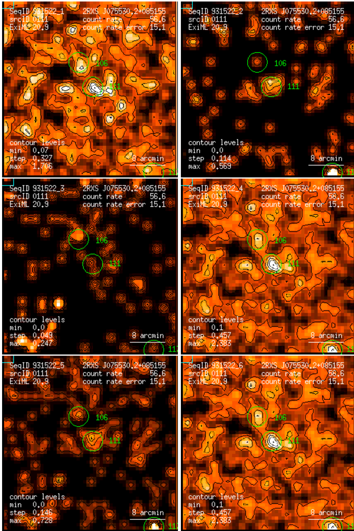
Figure 111: RASS 931522: detection 0111: band rate images, Gaussian filter: (1) PSPC channels 11 – 41, (2) 52 – 90, (3) 91 – 201, (4) 11 – 235, (5) 52 – 201, (6) 11 – 201. Broad band rates in counts/ks. Band rate contour levels in counts/ks/arcmin 2 .
