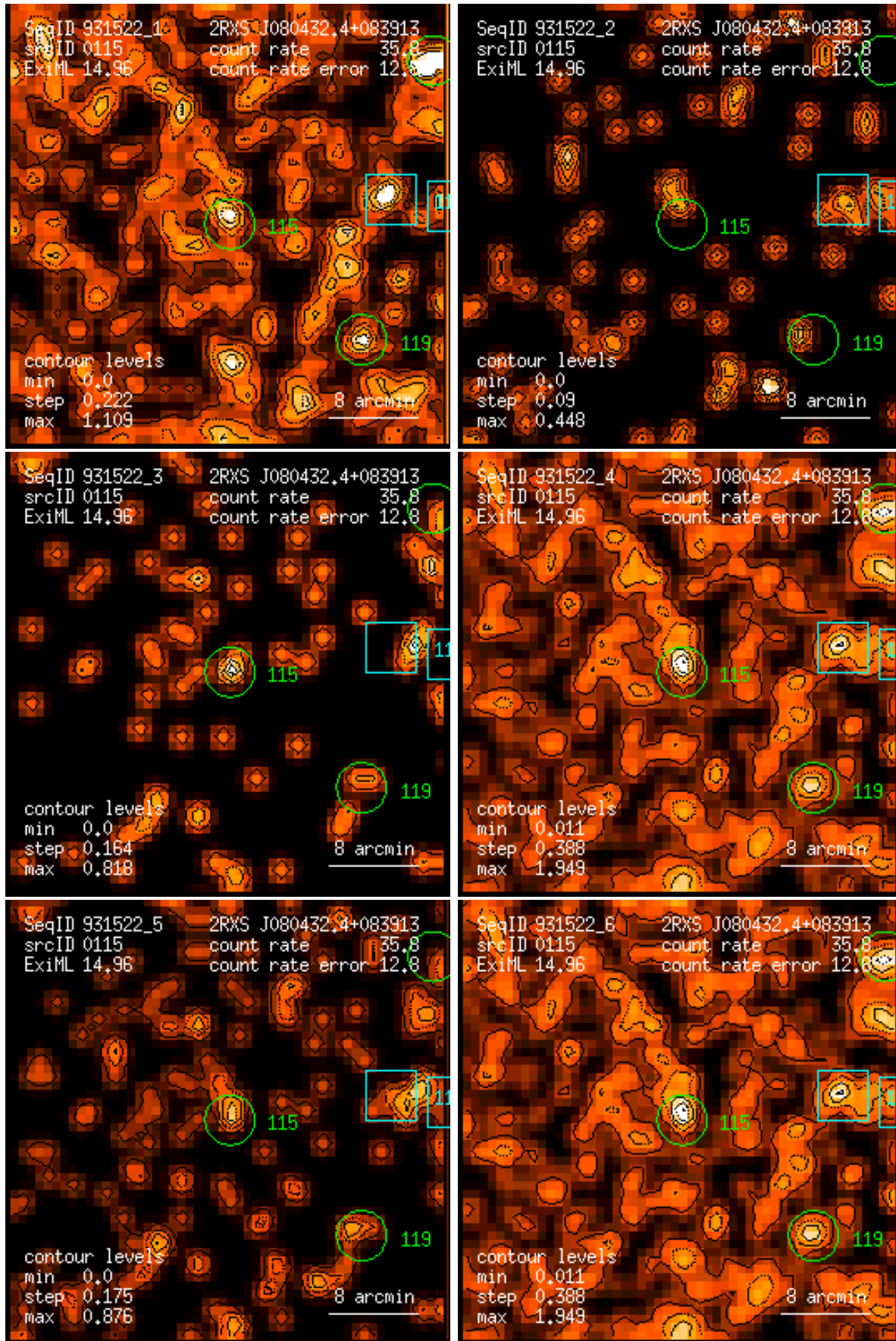
Figure 115: RASS 931522: detection 0115: band rate images, Gaussian filter: (1) PSPC channels 11 – 41, (2) 52 – 90, (3) 91 – 201, (4) 11 – 235, (5) 52 – 201, (6) 11 – 201. Broad band rates in counts/ks. Band rate contour levels in counts/ks/arcmin 2 .
