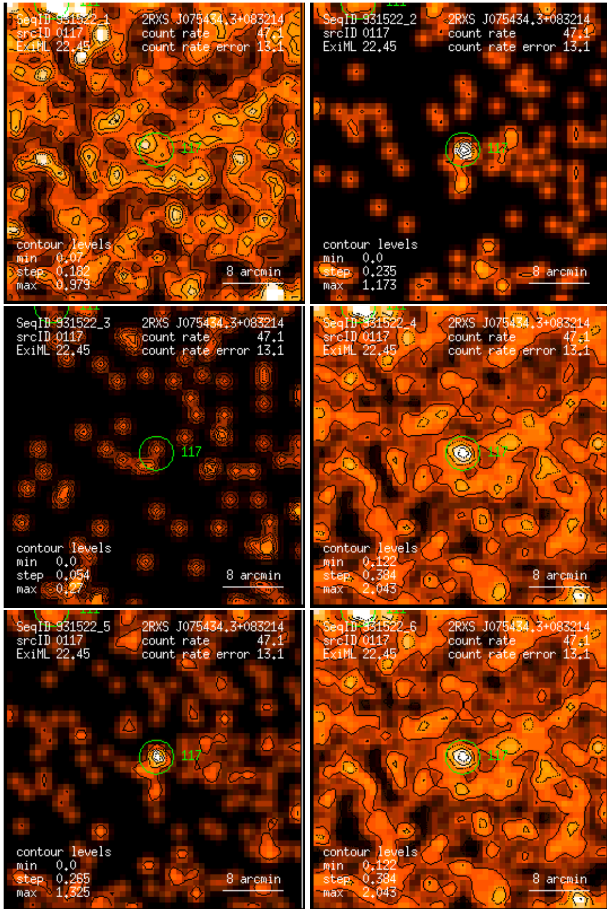
Figure 117: RASS 931522: detection 0117: band rate images, Gaussian filter: (1) PSPC channels 11 – 41, (2) 52 – 90, (3) 91 – 201, (4) 11 – 235, (5) 52 – 201, (6) 11 – 201. Broad band rates in counts/ks. Band rate contour levels in counts/ks/arcmin 2 .
