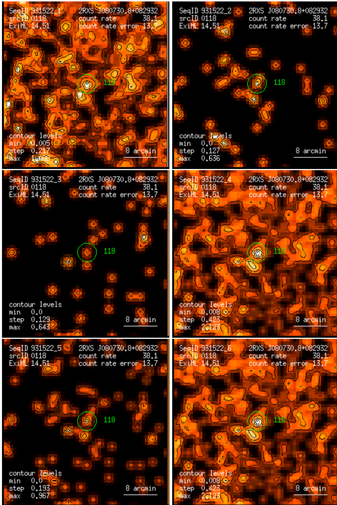
Figure 118: RASS 931522: detection 0118: band rate images, Gaussian filter: (1) PSPC channels 11 – 41, (2) 52 – 90, (3) 91 – 201, (4) 11 – 235, (5) 52 – 201, (6) 11 – 201. Broad band rates in counts/ks. Band rate contour levels in counts/ks/arcmin 2 .
