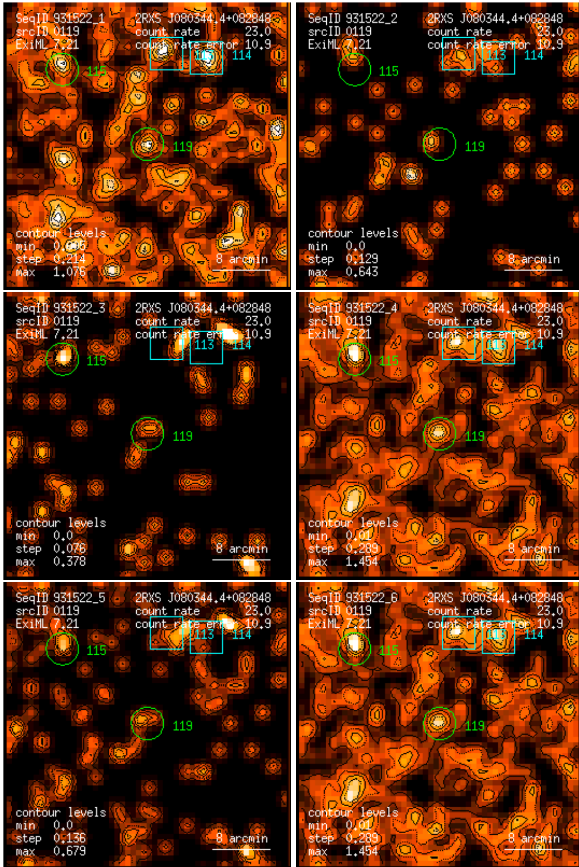
Figure 119: RASS 931522: detection 0119: band rate images, Gaussian filter: (1) PSPC channels 11 – 41, (2) 52 – 90, (3) 91 – 201, (4) 11 – 235, (5) 52 – 201, (6) 11 – 201. Broad band rates in counts/ks. Band rate contour levels in counts/ks/arcmin 2 .
