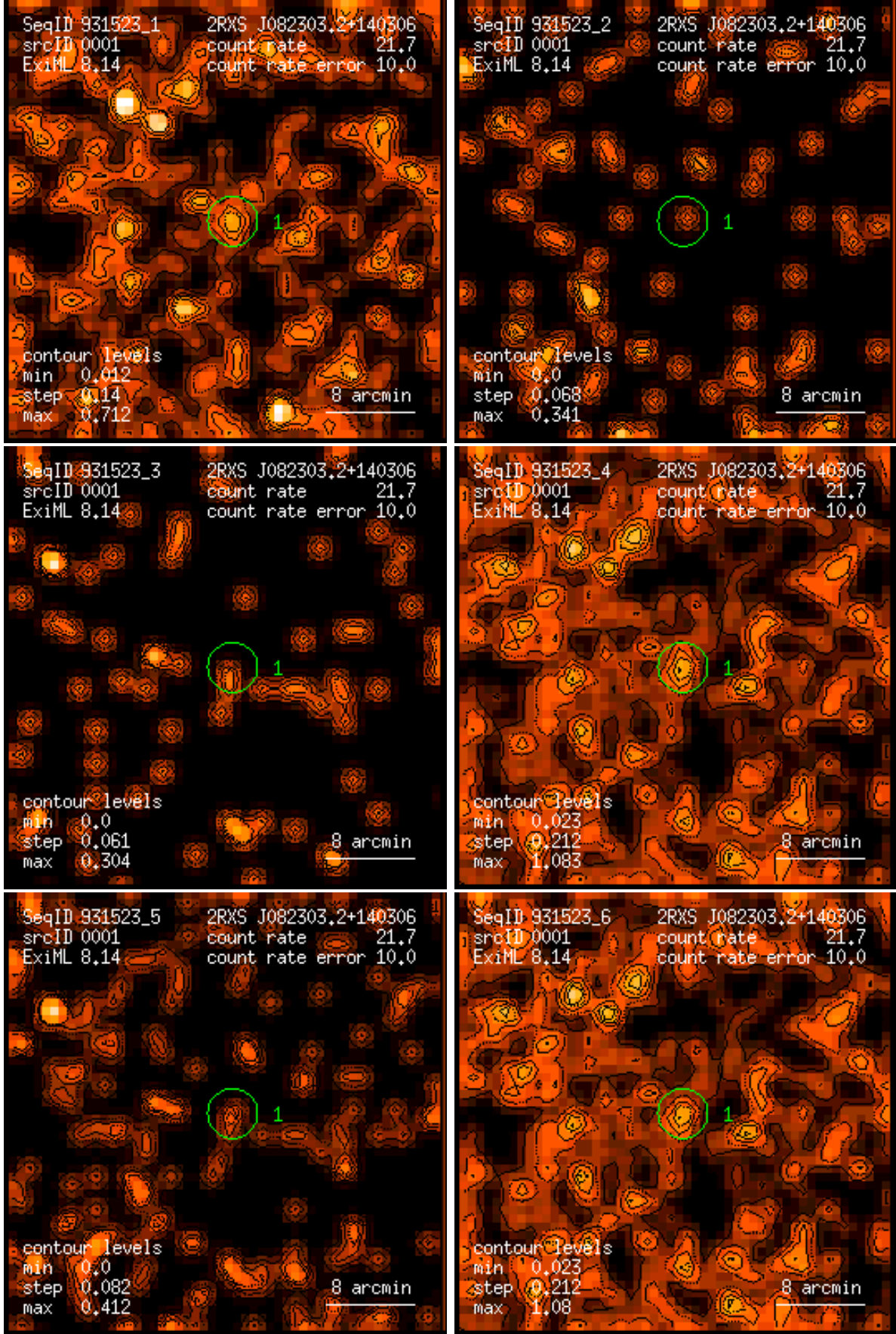
Figure 1: RASS 931523: detection 0001: band rate images, Gaussian filter: (1) PSPC channels 11 – 41, (2) 52 – 90, (3) 91 – 201, (4) 11 – 235, (5) 52 – 201, (6) 11 – 201. Broad band rates in counts/ks. Band rate contour levels in counts/ks/arcmin 2 .
