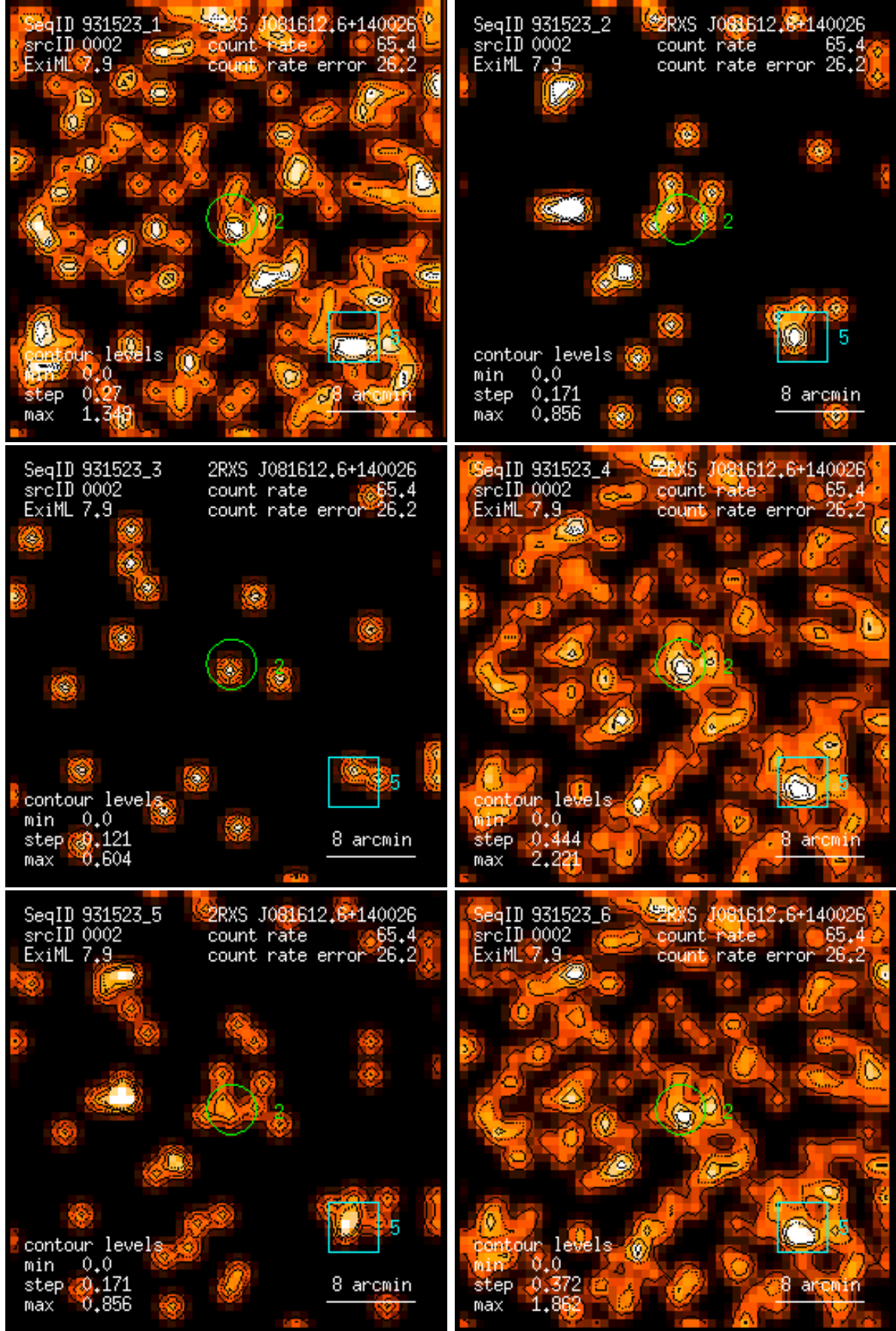
Figure 2: RASS 931523: detection 0002: band rate images, Gaussian filter: (1) PSPC channels 11 – 41, (2) 52 – 90, (3) 91 – 201, (4) 11 – 235, (5) 52 – 201, (6) 11 – 201. Broad band rates in counts/ks. Band rate contour levels in counts/ks/arcmin 2 .
