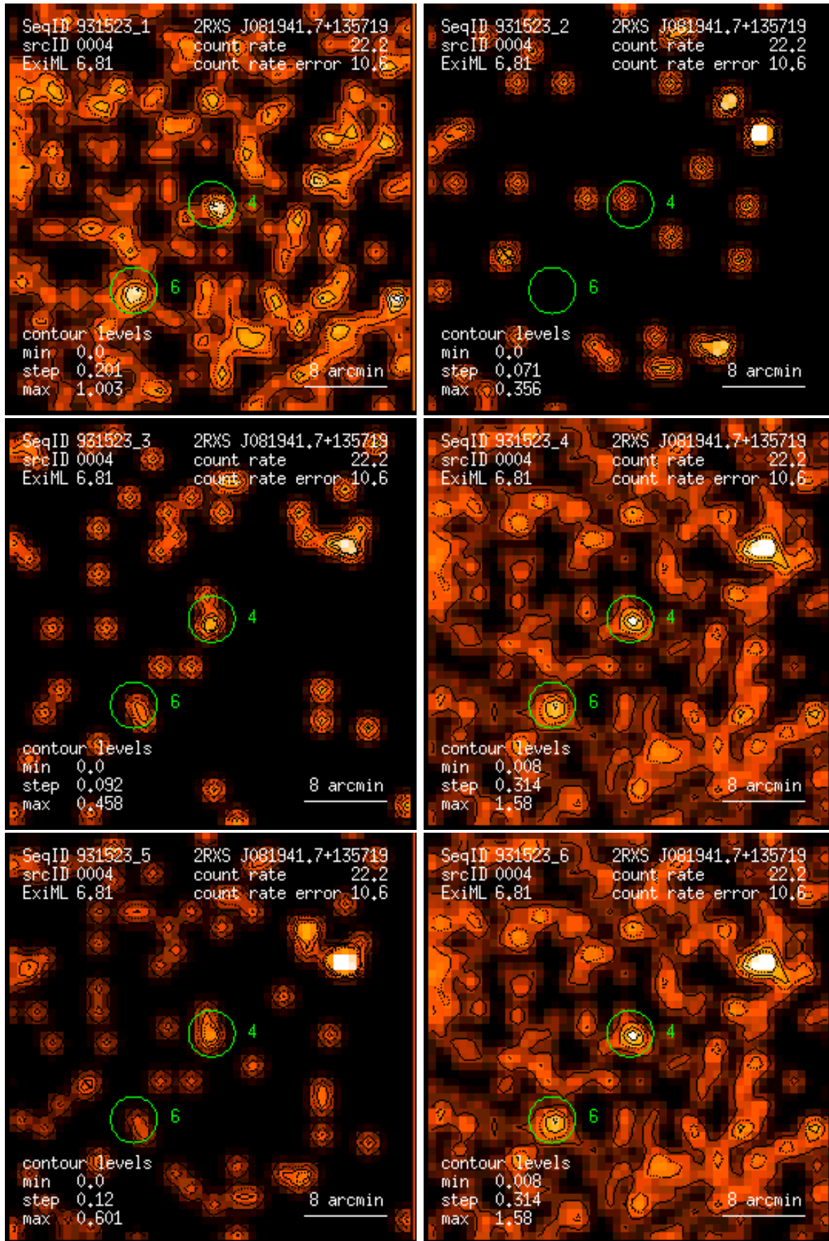
Figure 4: RASS 931523: detection 0004: band rate images, Gaussian filter: (1) PSPC channels 11 – 41, (2) 52 – 90, (3) 91 – 201, (4) 11 – 235, (5) 52 – 201, (6) 11 – 201. Broad band rates in counts/ks. Band rate contour levels in counts/ks/arcmin 2 .
