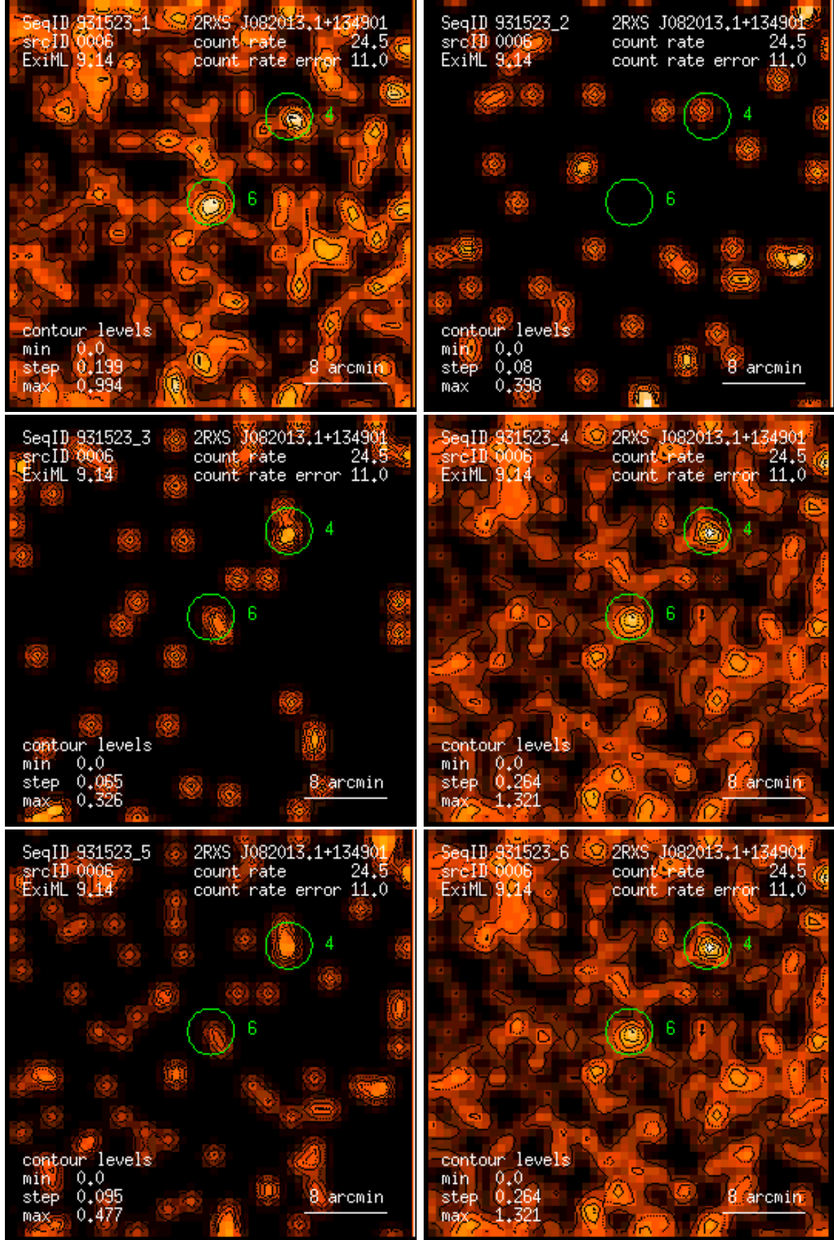
Figure 6: RASS 931523: detection 0006: band rate images, Gaussian filter: (1) PSPC channels 11 – 41, (2) 52 – 90, (3) 91 – 201, (4) 11 – 235, (5) 52 – 201, (6) 11 – 201. Broad band rates in counts/ks. Band rate contour levels in counts/ks/arcmin 2 .
