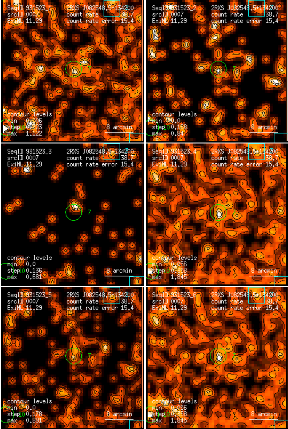
Figure 7: RASS 931523: detection 0007: band rate images, Gaussian filter: (1) PSPC channels 11 – 41, (2) 52 – 90, (3) 91 – 201, (4) 11 – 235, (5) 52 – 201, (6) 11 – 201. Broad band rates in counts/ks. Band rate contour levels in counts/ks/arcmin 2 .
