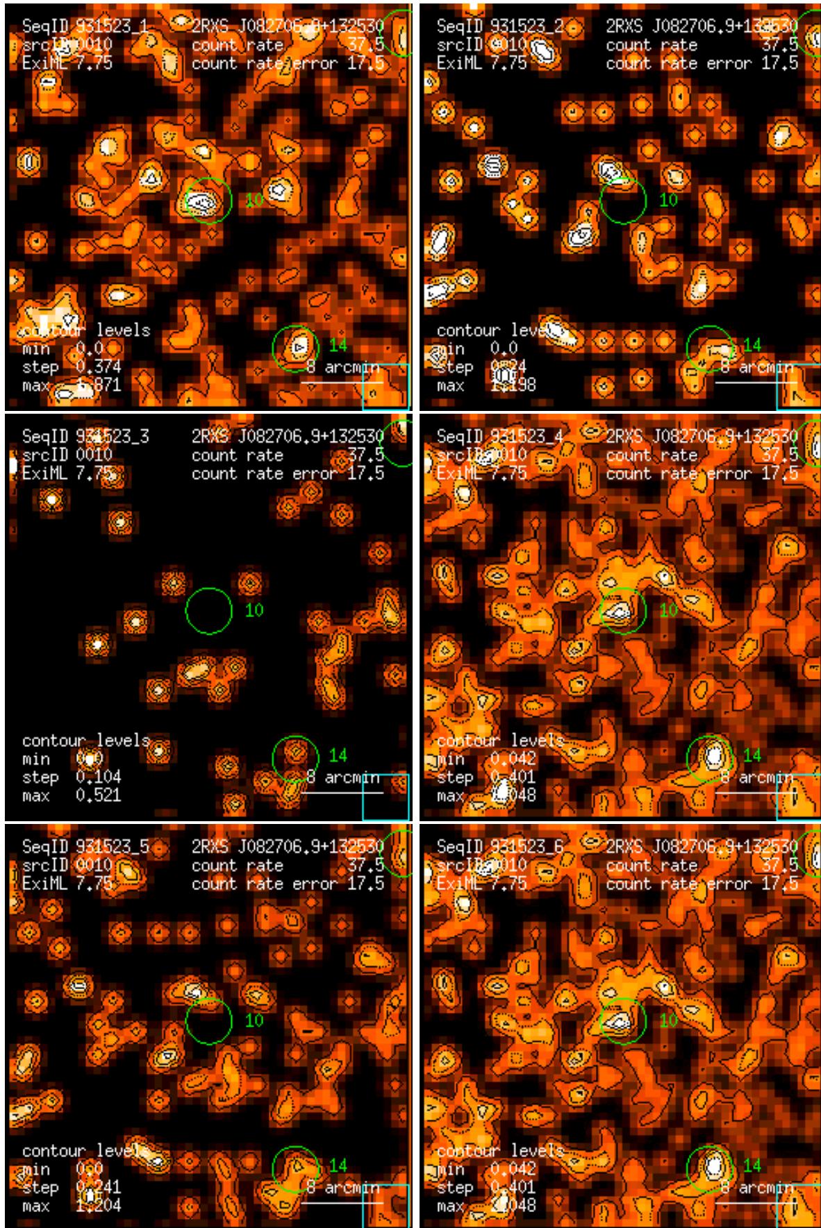
Figure 10: RASS 931523: detection 0010: band rate images, Gaussian filter: (1) PSPC channels 11 – 41, (2) 52 – 90, (3) 91 – 201, (4) 11 – 235, (5) 52 – 201, (6) 11 – 201. Broad band rates in counts/ks. Band rate contour levels in counts/ks/arcmin 2 .
