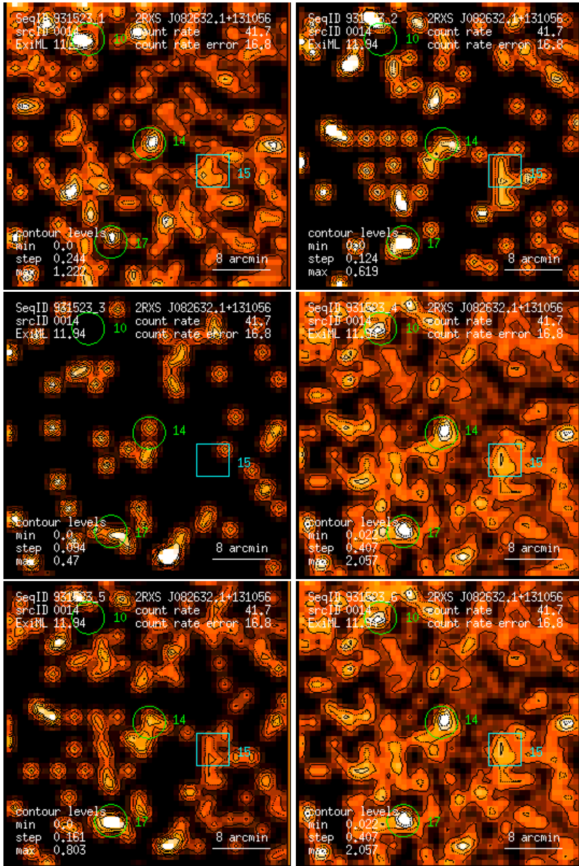
Figure 14: RASS 931523: detection 0014: band rate images, Gaussian filter: (1) PSPC channels 11 – 41, (2) 52 – 90, (3) 91 – 201, (4) 11 – 235, (5) 52 – 201, (6) 11 – 201. Broad band rates in counts/ks. Band rate contour levels in counts/ks/arcmin 2 .
