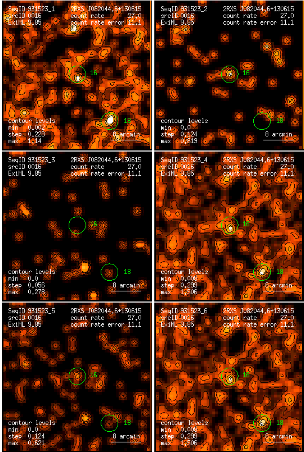
Figure 16: RASS 931523: detection 0016: band rate images, Gaussian filter: (1) PSPC channels 11 – 41, (2) 52 – 90, (3) 91 – 201, (4) 11 – 235, (5) 52 – 201, (6) 11 – 201. Broad band rates in counts/ks. Band rate contour levels in counts/ks/arcmin 2 .
