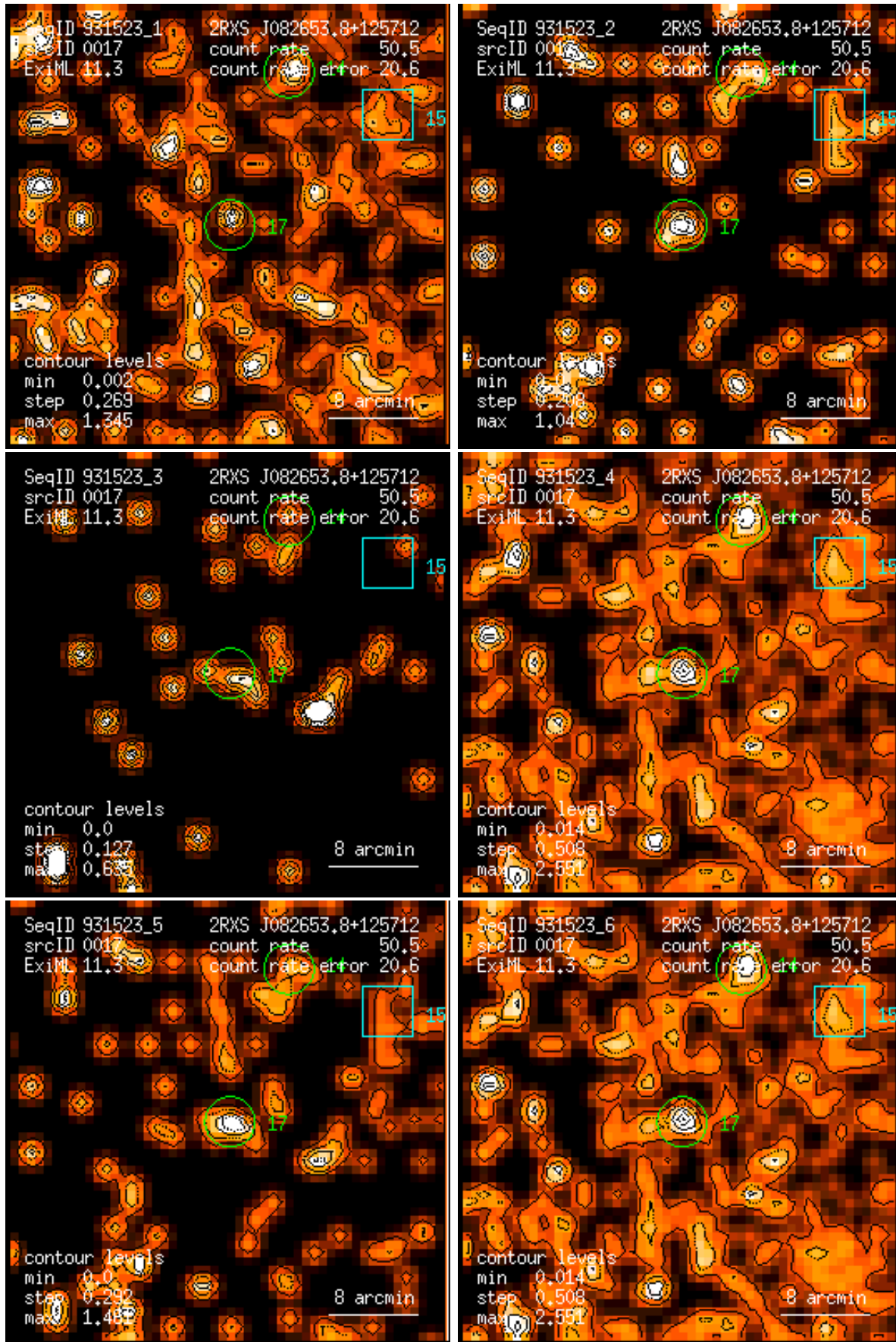
Figure 17: RASS 931523: detection 0017: band rate images, Gaussian filter: (1) PSPC channels 11 – 41, (2) 52 – 90, (3) 91 – 201, (4) 11 – 235, (5) 52 – 201, (6) 11 – 201. Broad band rates in counts/ks. Band rate contour levels in counts/ks/arcmin 2 .
