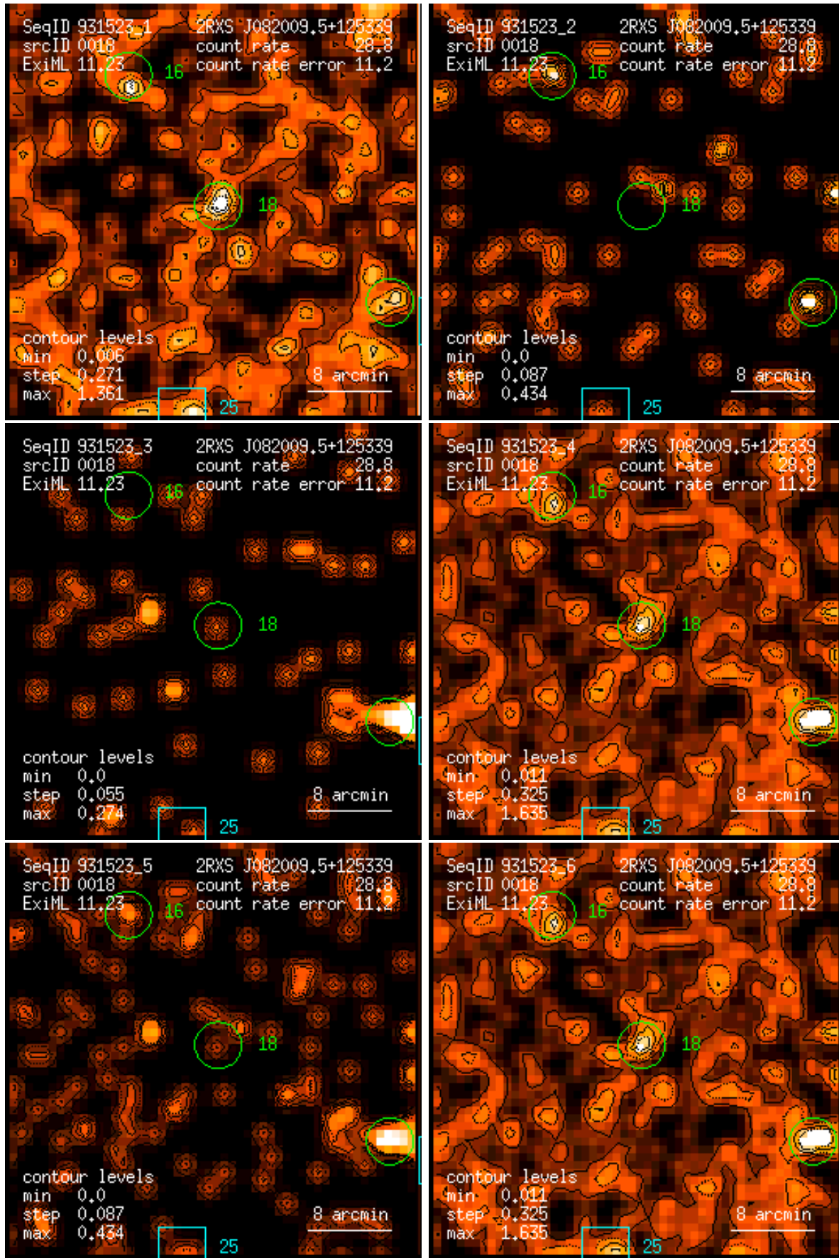
Figure 18: RASS 931523: detection 0018: band rate images, Gaussian filter: (1) PSPC channels 11 – 41, (2) 52 – 90, (3) 91 – 201, (4) 11 – 235, (5) 52 – 201, (6) 11 – 201. Broad band rates in counts/ks. Band rate contour levels in counts/ks/arcmin 2 .
