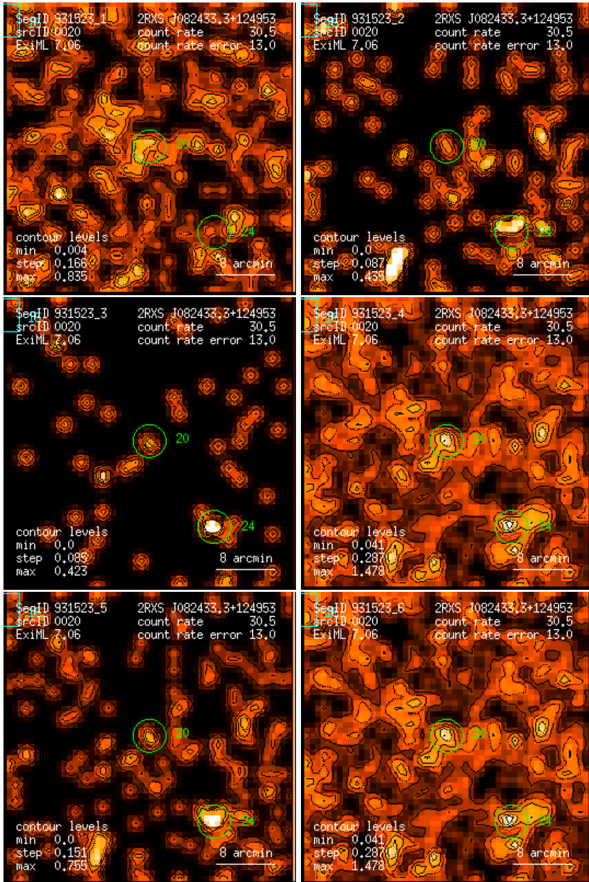
Figure 20: RASS 931523: detection 0020: band rate images, Gaussian filter: (1) PSPC channels 11 – 41, (2) 52 – 90, (3) 91 – 201, (4) 11 – 235, (5) 52 – 201, (6) 11 – 201. Broad band rates in counts/ks. Band rate contour levels in counts/ks/arcmin 2 .
