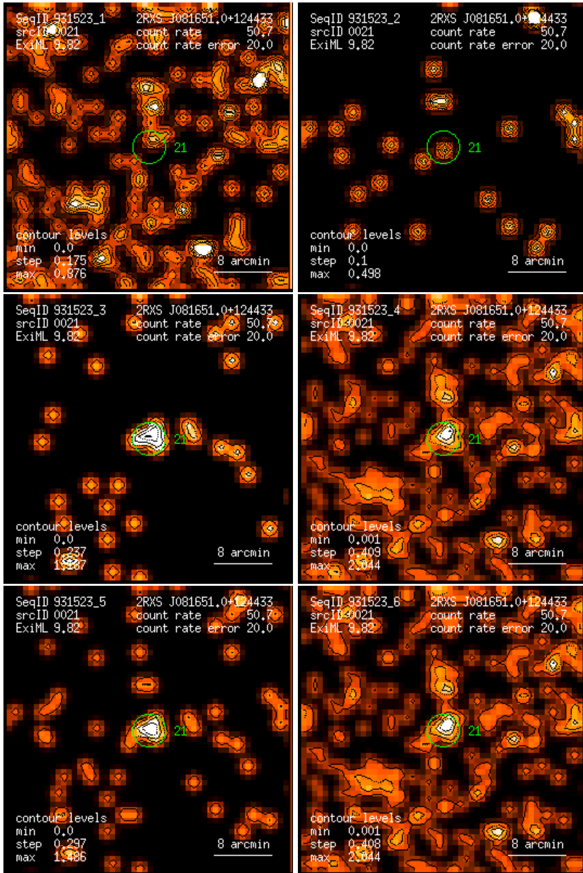
Figure 21: RASS 931523: detection 0021: band rate images, Gaussian filter: (1) PSPC channels 11 – 41, (2) 52 – 90, (3) 91 – 201, (4) 11 – 235, (5) 52 – 201, (6) 11 – 201. Broad band rates in counts/ks. Band rate contour levels in counts/ks/arcmin 2 .
