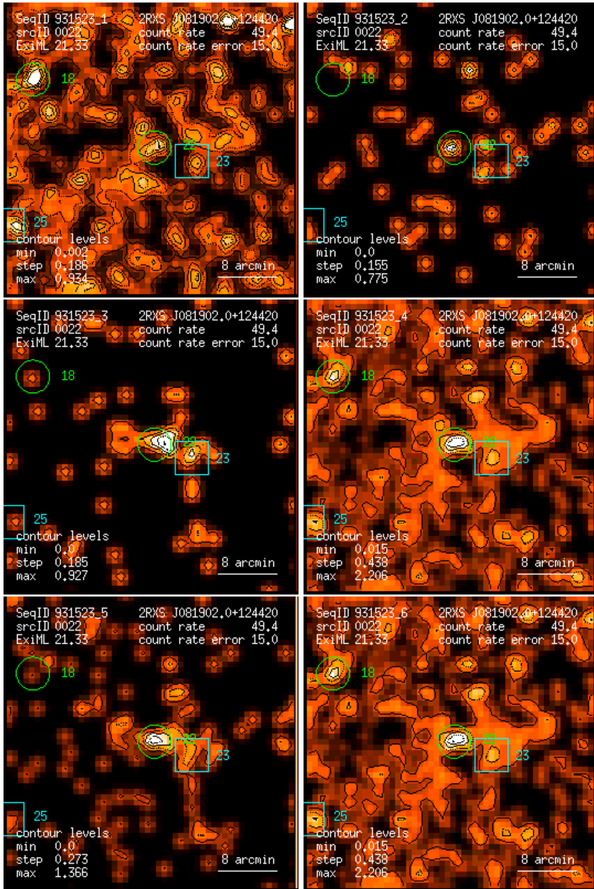
Figure 22: RASS 931523: detection 0022: band rate images, Gaussian filter: (1) PSPC channels 11 – 41, (2) 52 – 90, (3) 91 – 201, (4) 11 – 235, (5) 52 – 201, (6) 11 – 201. Broad band rates in counts/ks. Band rate contour levels in counts/ks/arcmin 2 .
