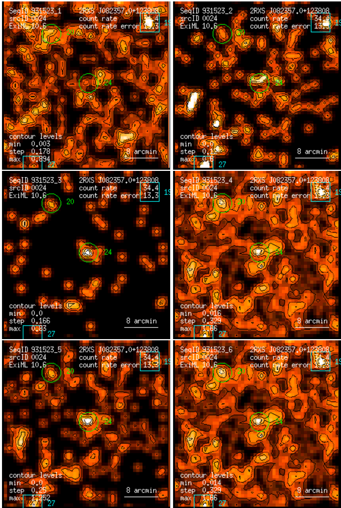
Figure 24: RASS 931523: detection 0024: band rate images, Gaussian filter: (1) PSPC channels 11 – 41, (2) 52 – 90, (3) 91 – 201, (4) 11 – 235, (5) 52 – 201, (6) 11 – 201. Broad band rates in counts/ks. Band rate contour levels in counts/ks/arcmin 2 .
