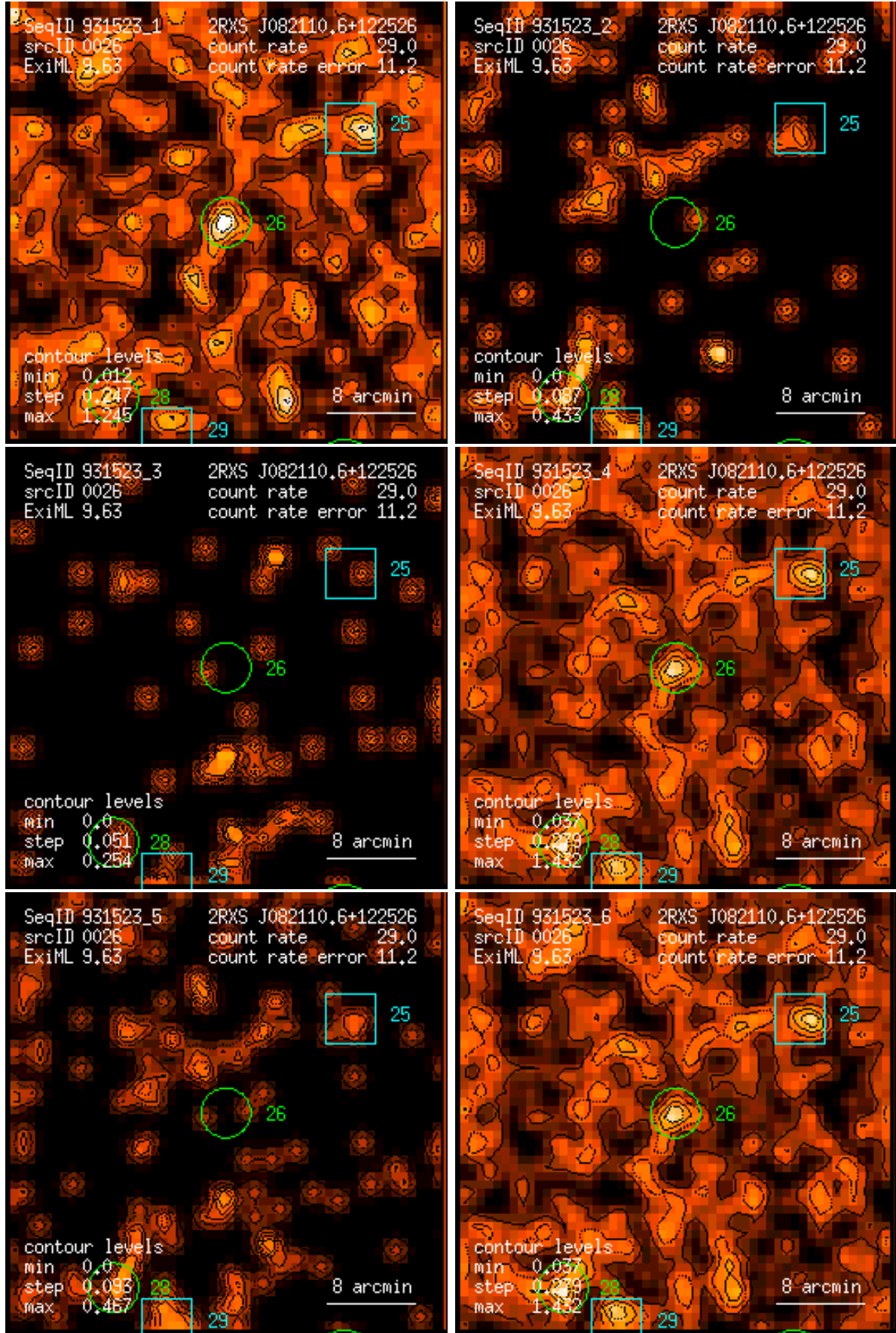
Figure 26: RASS 931523: detection 0026: band rate images, Gaussian filter: (1) PSPC channels 11 – 41, (2) 52 – 90, (3) 91 – 201, (4) 11 – 235, (5) 52 – 201, (6) 11 – 201. Broad band rates in counts/ks. Band rate contour levels in counts/ks/arcmin 2 .
