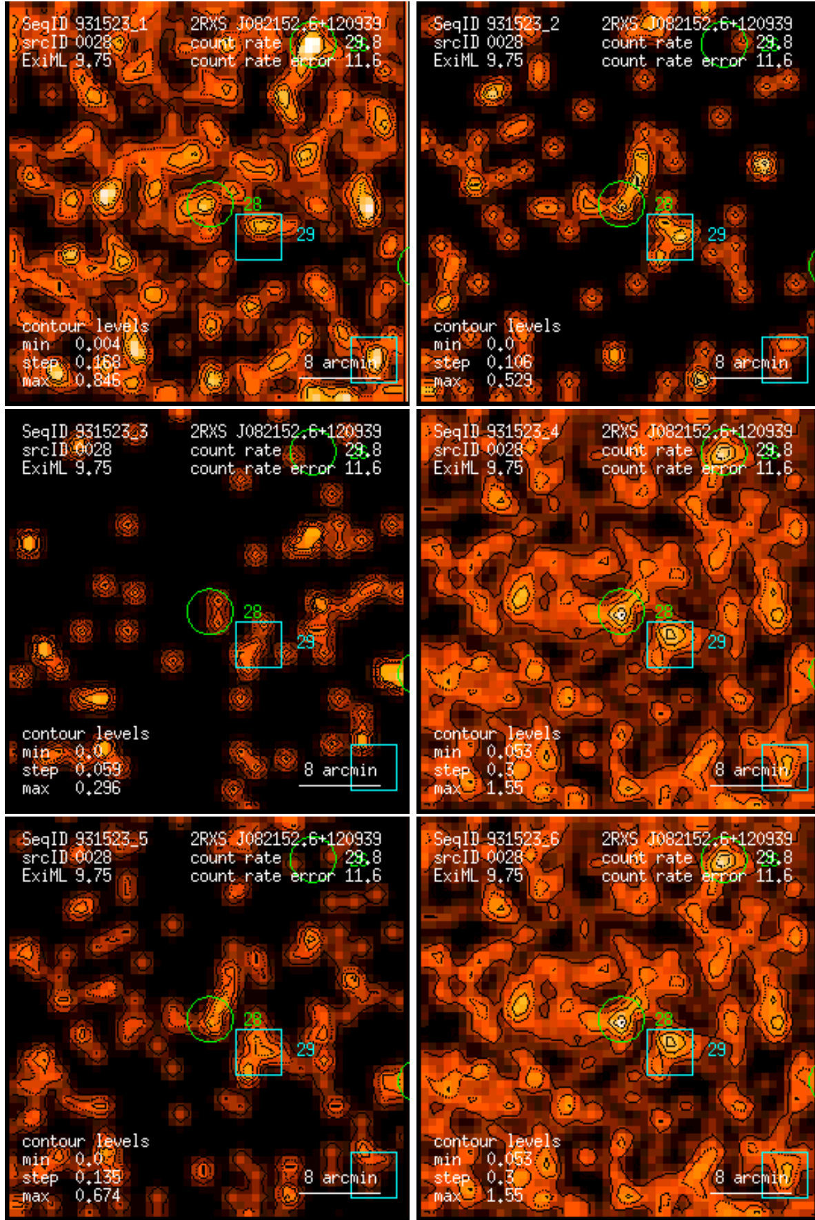
Figure 28: RASS 931523: detection 0028: band rate images, Gaussian filter: (1) PSPC channels 11 – 41, (2) 52 – 90, (3) 91 – 201, (4) 11 – 235, (5) 52 – 201, (6) 11 – 201. Broad band rates in counts/ks. Band rate contour levels in counts/ks/arcmin 2 .
