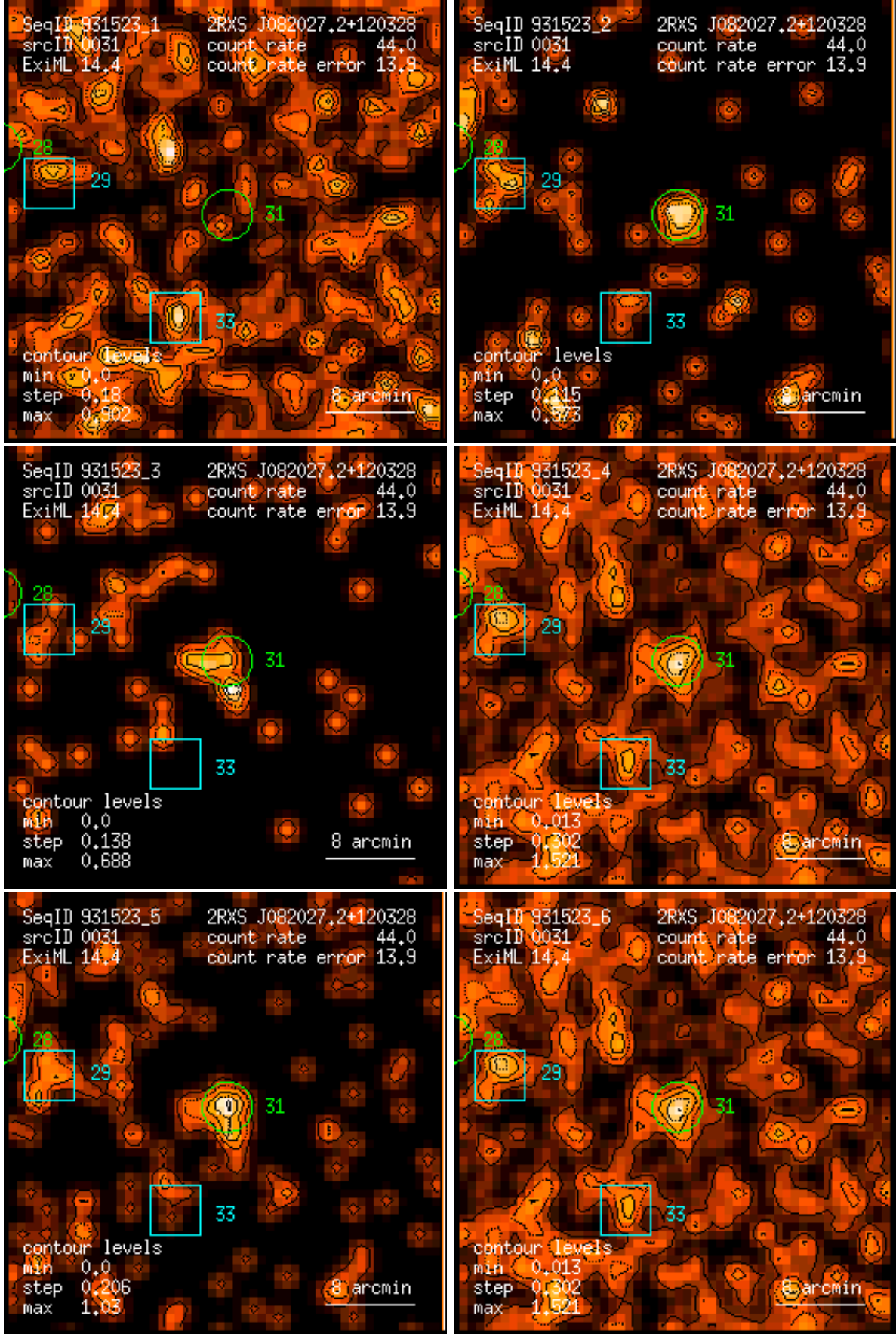
Figure 31: RASS 931523: detection 0031: band rate images, Gaussian filter: (1) PSPC channels 11 – 41, (2) 52 – 90, (3) 91 – 201, (4) 11 – 235, (5) 52 – 201, (6) 11 – 201. Broad band rates in counts/ks. Band rate contour levels in counts/ks/arcmin 2 .
