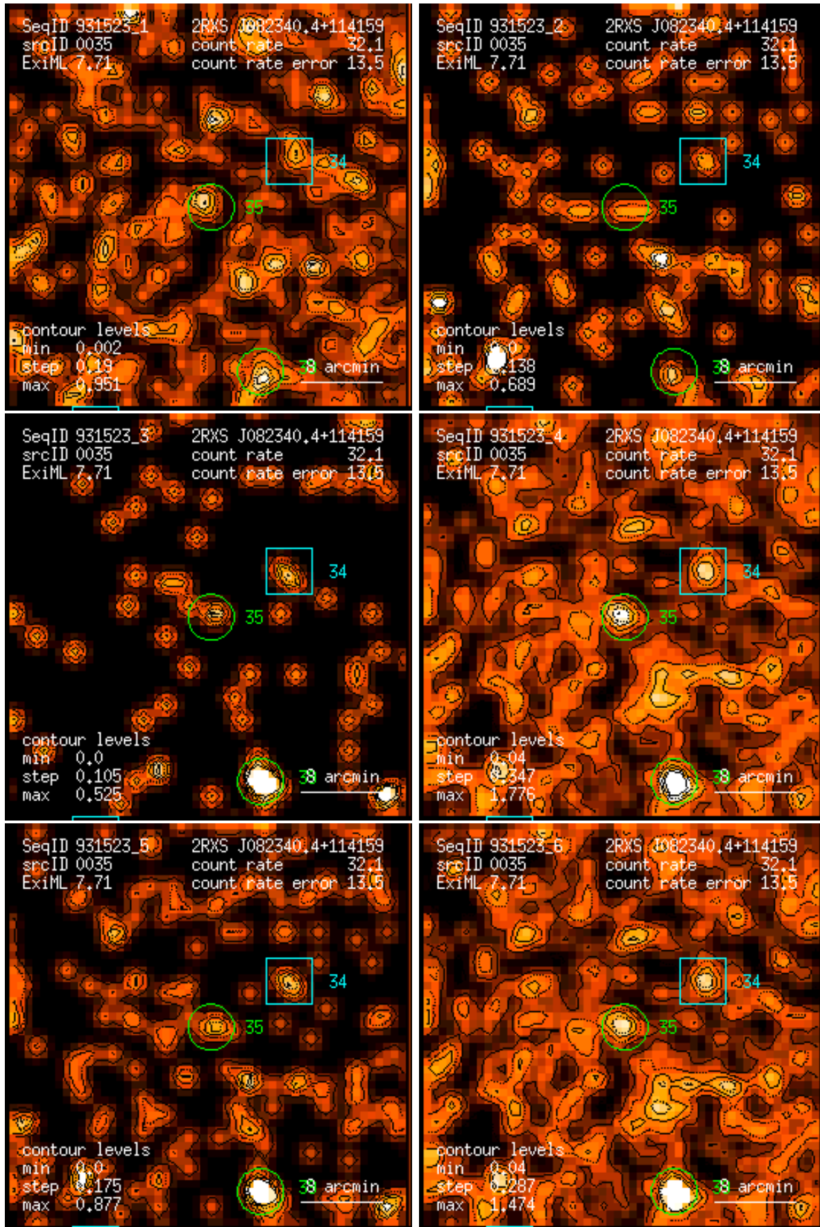
Figure 35: RASS 931523: detection 0035: band rate images, Gaussian filter: (1) PSPC channels 11 – 41, (2) 52 – 90, (3) 91 – 201, (4) 11 – 235, (5) 52 – 201, (6) 11 – 201. Broad band rates in counts/ks. Band rate contour levels in counts/ks/arcmin 2 .
