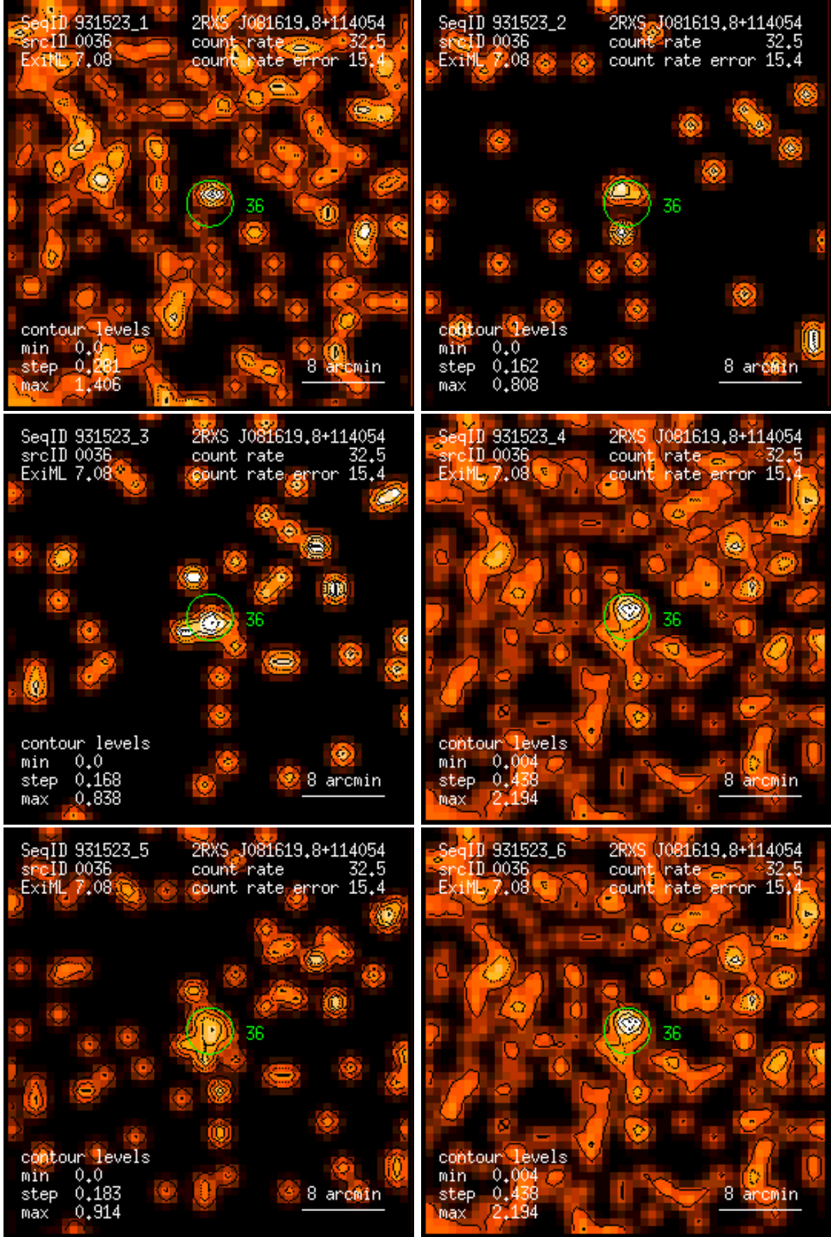
Figure 36: RASS 931523: detection 0036: band rate images, Gaussian filter: (1) PSPC channels 11 – 41, (2) 52 – 90, (3) 91 – 201, (4) 11 – 235, (5) 52 – 201, (6) 11 – 201. Broad band rates in counts/ks. Band rate contour levels in counts/ks/arcmin 2 .
