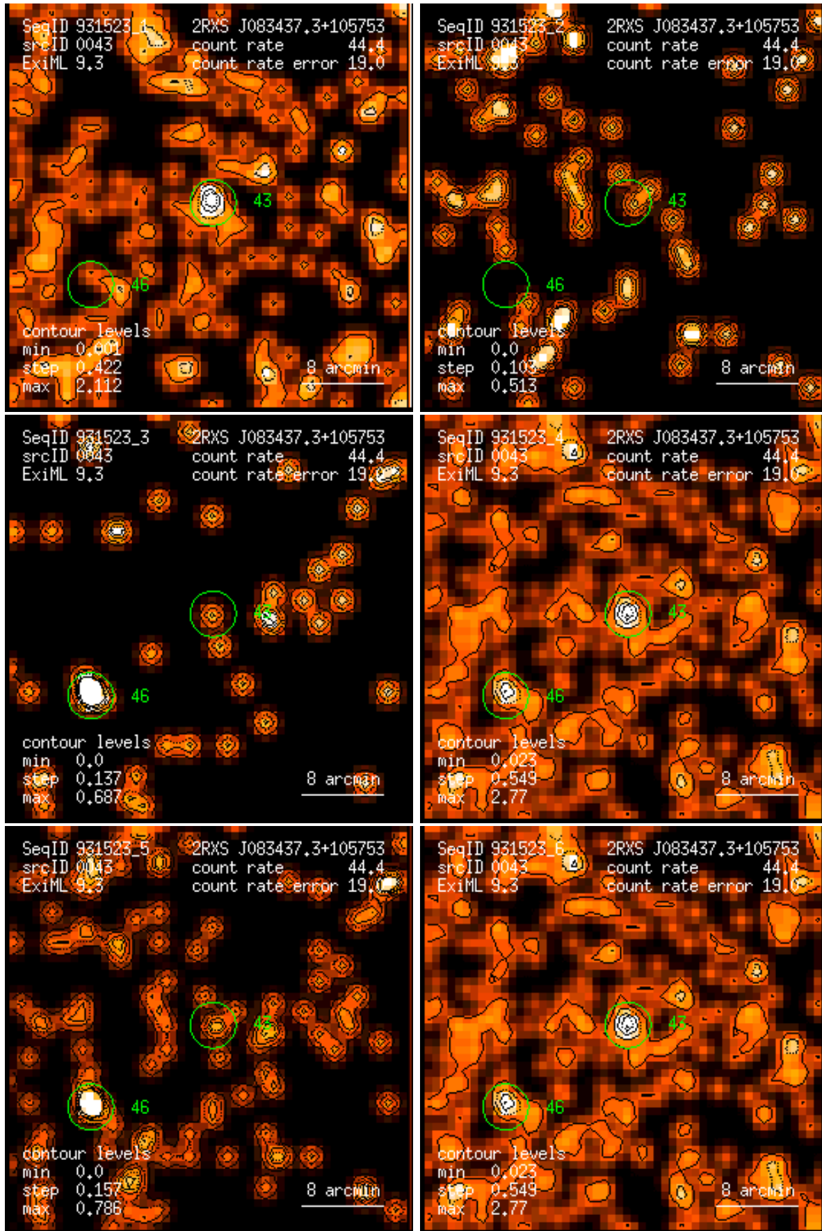
Figure 43: RASS 931523: detection 0043: band rate images, Gaussian filter: (1) PSPC channels 11 – 41, (2) 52 – 90, (3) 91 – 201, (4) 11 – 235, (5) 52 – 201, (6) 11 – 201. Broad band rates in counts/ks. Band rate contour levels in counts/ks/arcmin 2 .
