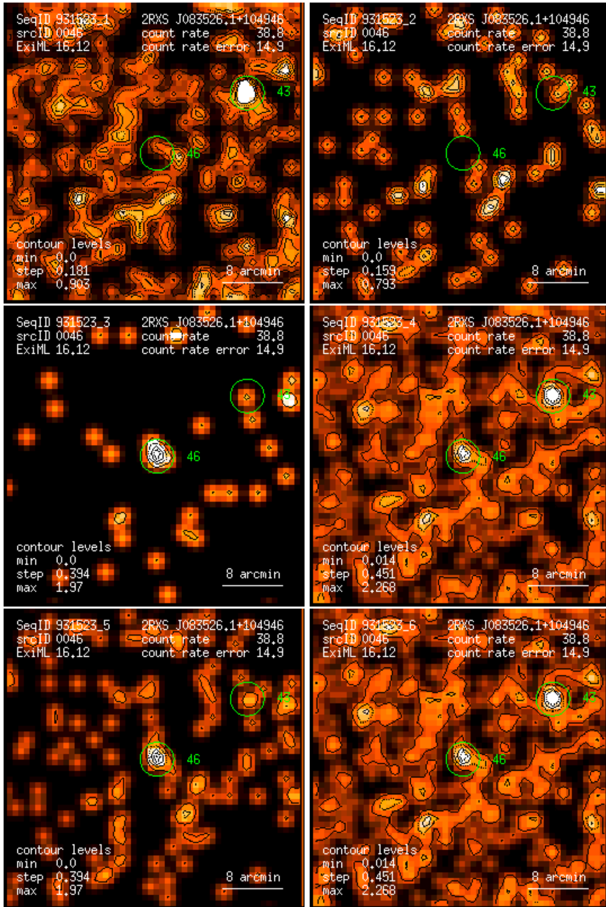
Figure 46: RASS 931523: detection 0046: band rate images, Gaussian filter: (1) PSPC channels 11 – 41, (2) 52 – 90, (3) 91 – 201, (4) 11 – 235, (5) 52 – 201, (6) 11 – 201. Broad band rates in counts/ks. Band rate contour levels in counts/ks/arcmin 2 .
