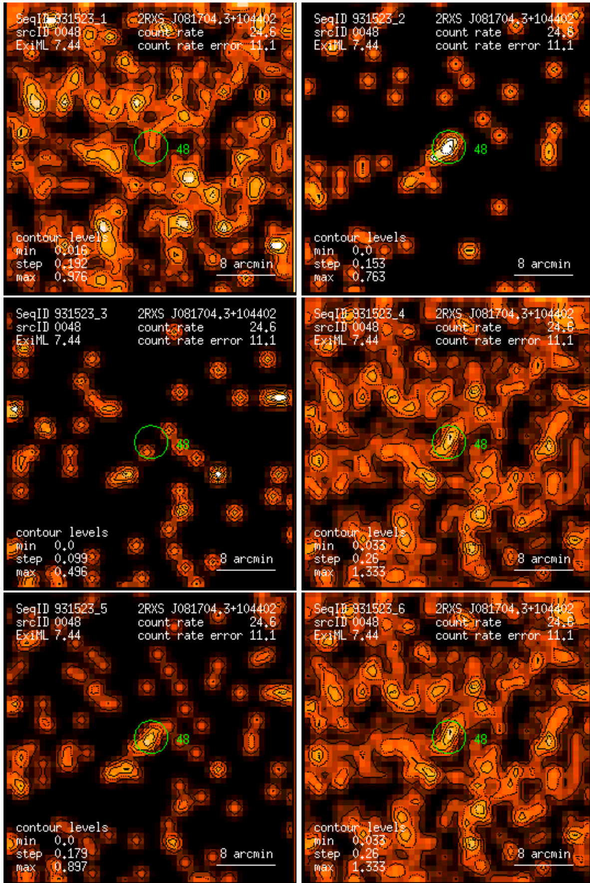
Figure 48: RASS 931523: detection 0048: band rate images, Gaussian filter: (1) PSPC channels 11 – 41, (2) 52 – 90, (3) 91 – 201, (4) 11 – 235, (5) 52 – 201, (6) 11 – 201. Broad band rates in counts/ks. Band rate contour levels in counts/ks/arcmin 2 .
