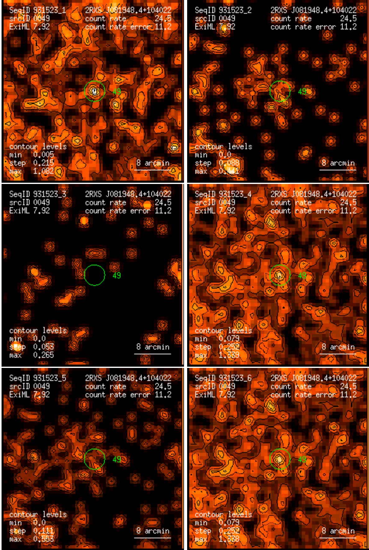
Figure 49: RASS 931523: detection 0049: band rate images, Gaussian filter: (1) PSPC channels 11 – 41, (2) 52 – 90, (3) 91 – 201, (4) 11 – 235, (5) 52 – 201, (6) 11 – 201. Broad band rates in counts/ks. Band rate contour levels in counts/ks/arcmin 2 .
