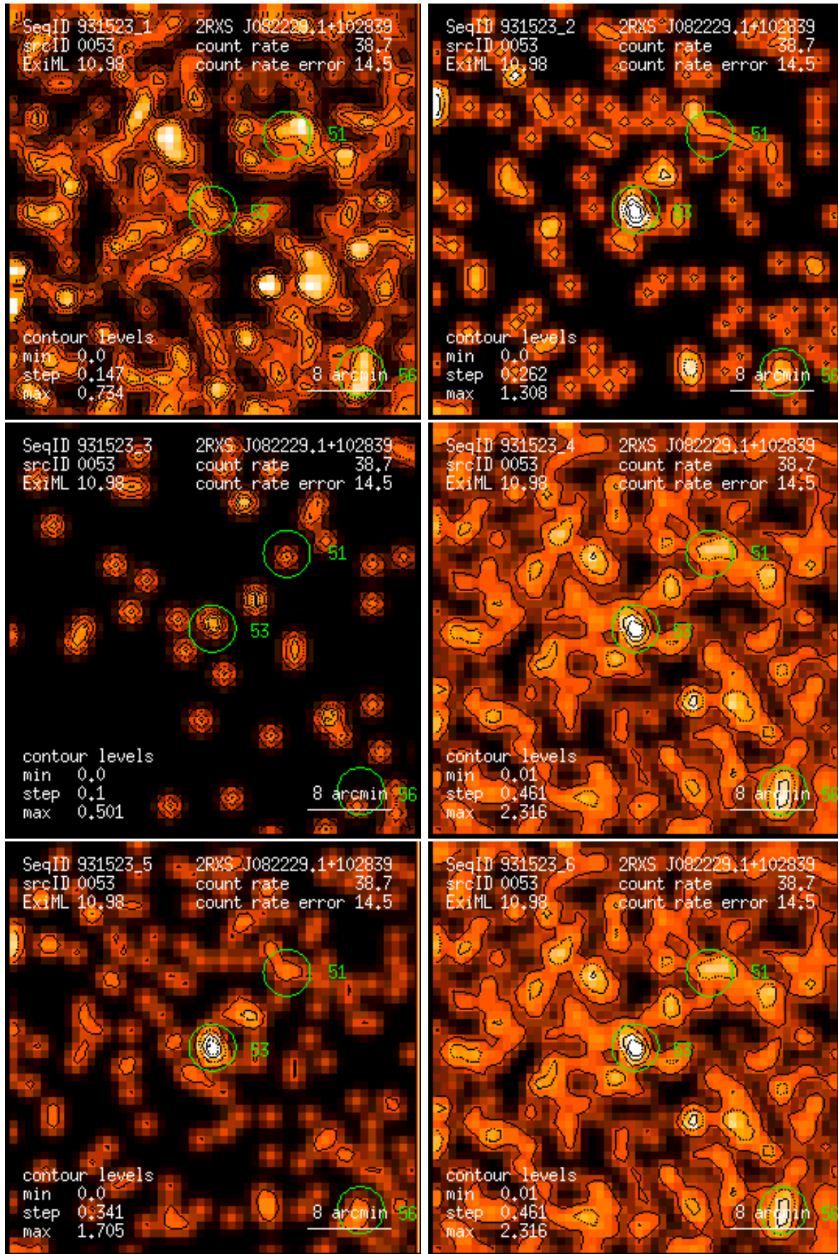
Figure 53: RASS 931523: detection 0053: band rate images, Gaussian filter: (1) PSPC channels 11 – 41, (2) 52 – 90, (3) 91 – 201, (4) 11 – 235, (5) 52 – 201, (6) 11 – 201. Broad band rates in counts/ks. Band rate contour levels in counts/ks/arcmin 2 .
