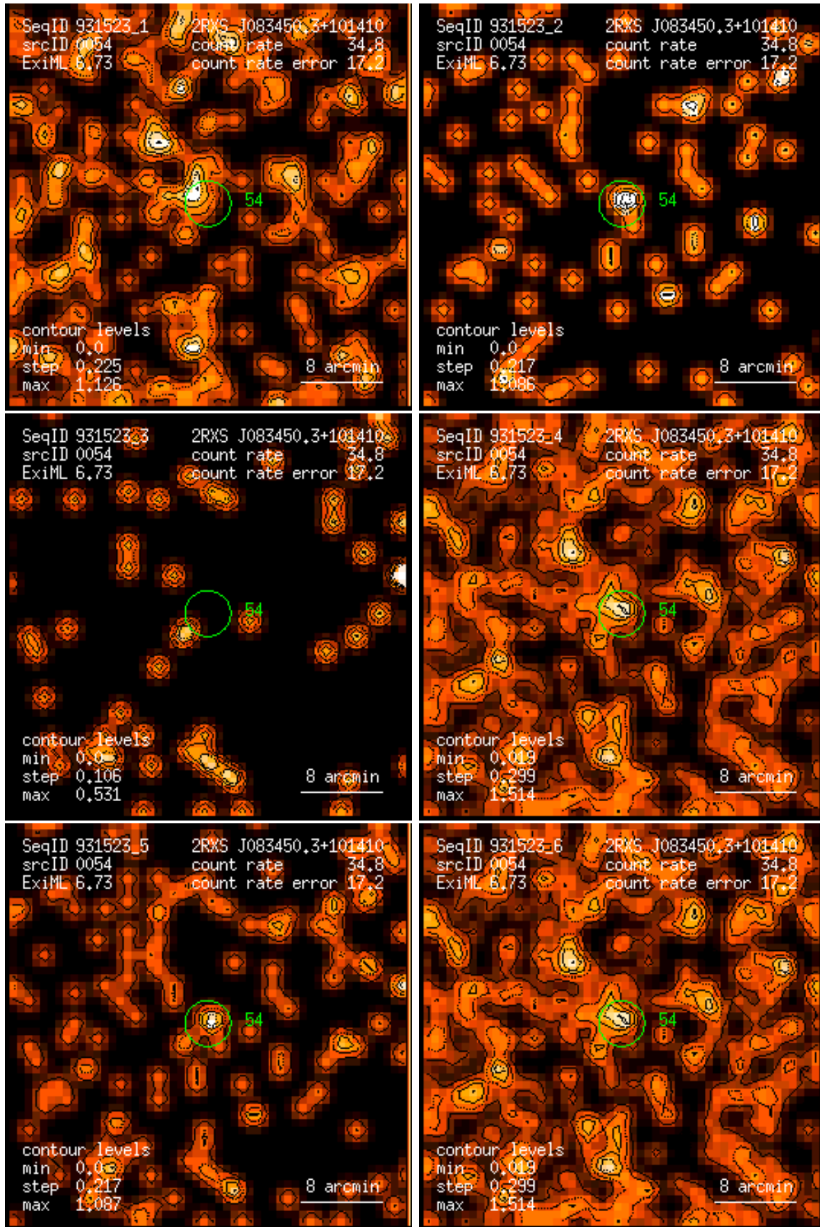
Figure 54: RASS 931523: detection 0054: band rate images, Gaussian filter: (1) PSPC channels 11 – 41, (2) 52 – 90, (3) 91 – 201, (4) 11 – 235, (5) 52 – 201, (6) 11 – 201. Broad band rates in counts/ks. Band rate contour levels in counts/ks/arcmin 2 .
