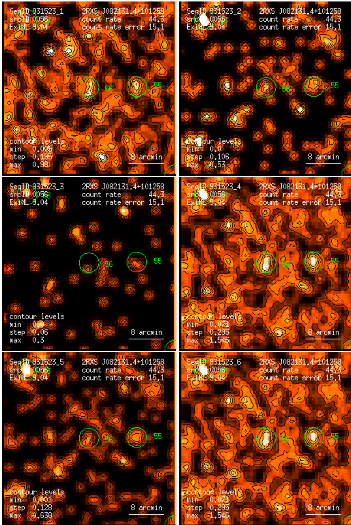
Figure 56: RASS 931523: detection 0056: band rate images, Gaussian filter: (1) PSPC channels 11 – 41, (2) 52 – 90, (3) 91 – 201, (4) 11 – 235, (5) 52 – 201, (6) 11 – 201. Broad band rates in counts/ks. Band rate contour levels in counts/ks/arcmin 2 .
