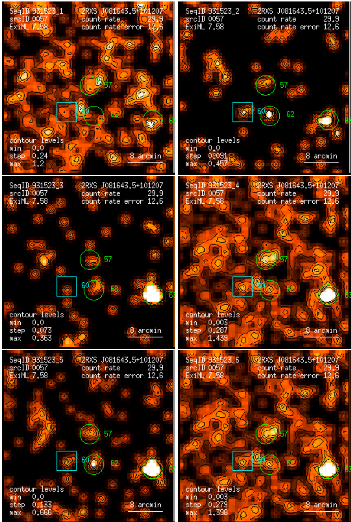
Figure 57: RASS 931523: detection 0057: band rate images, Gaussian filter: (1) PSPC channels 11 – 41, (2) 52 – 90, (3) 91 – 201, (4) 11 – 235, (5) 52 – 201, (6) 11 – 201. Broad band rates in counts/ks. Band rate contour levels in counts/ks/arcmin 2 .
