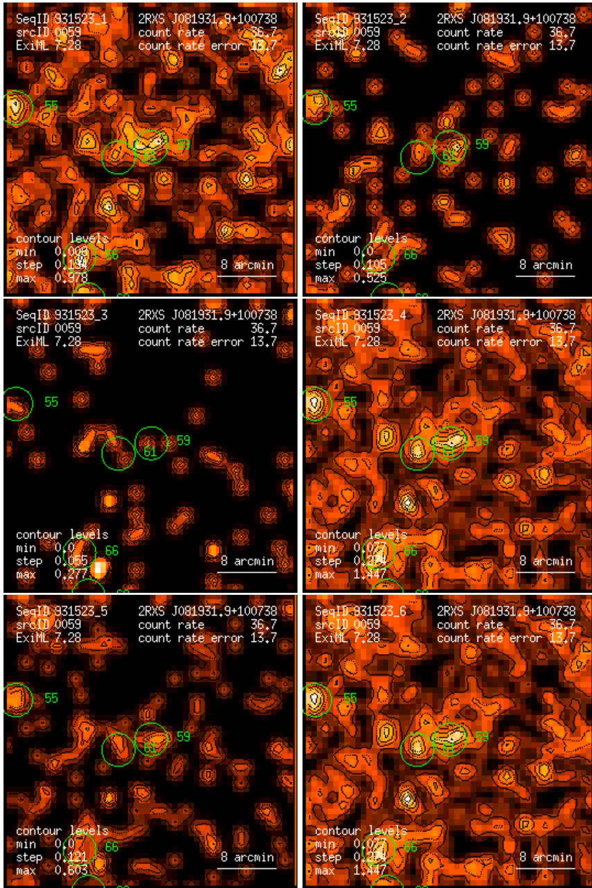
Figure 59: RASS 931523: detection 0059: band rate images, Gaussian filter: (1) PSPC channels 11 – 41, (2) 52 – 90, (3) 91 – 201, (4) 11 – 235, (5) 52 – 201, (6) 11 – 201. Broad band rates in counts/ks. Band rate contour levels in counts/ks/arcmin 2 .
